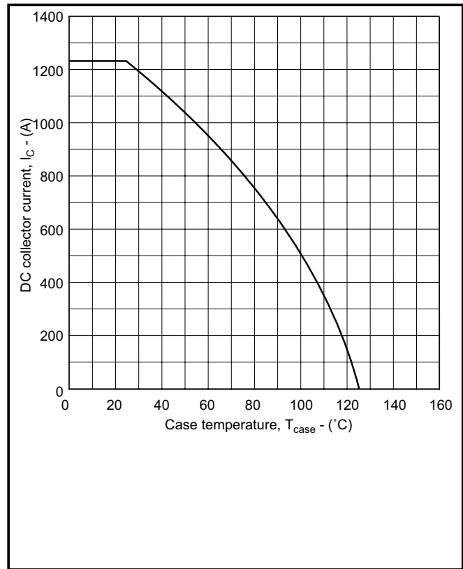
Fig. 15 DC current rating vs case temperature
