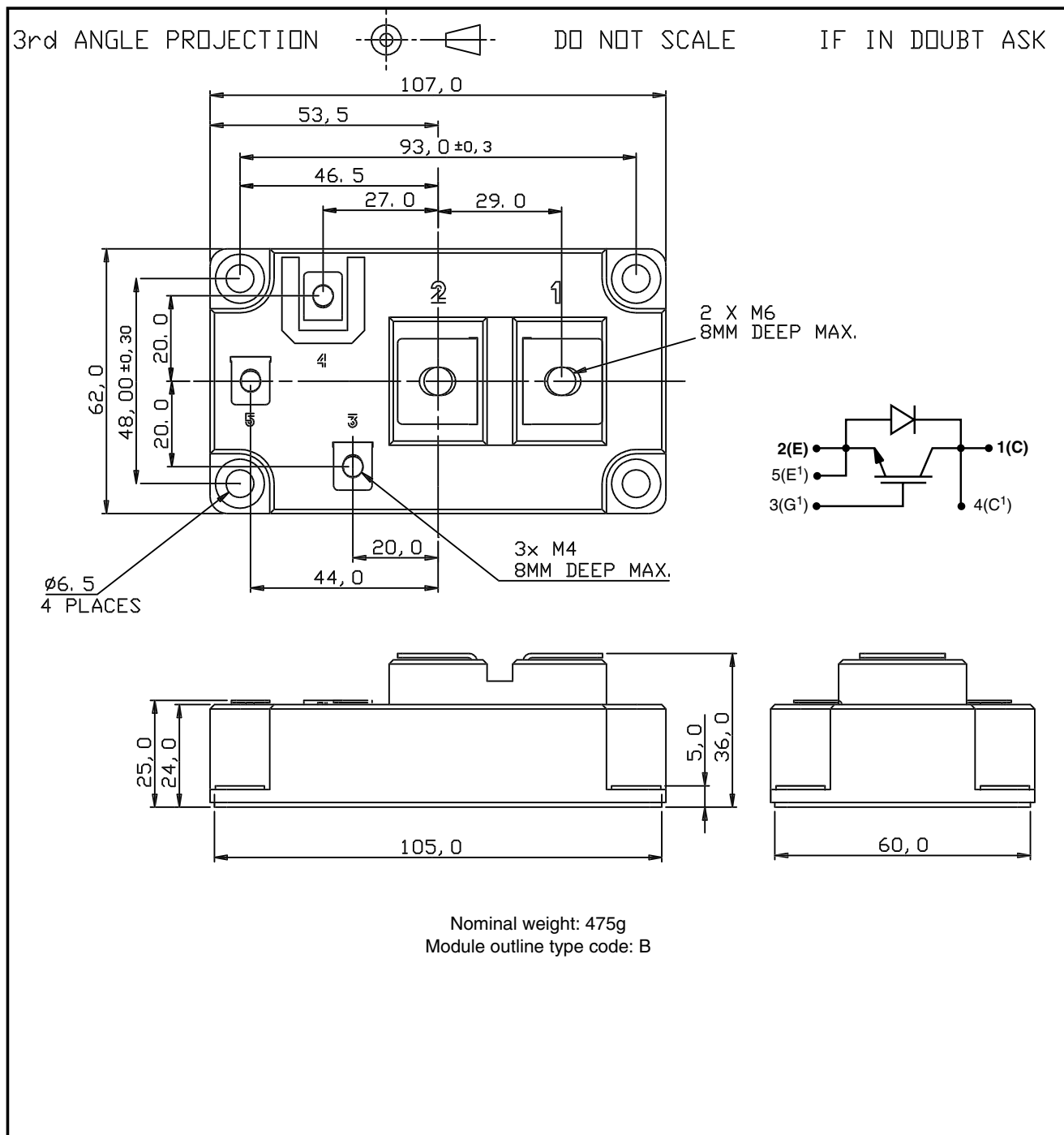
Fig. 11 Package details
