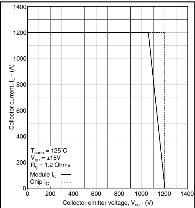
Fig. 8 IGBT reverse bias safe operating area
