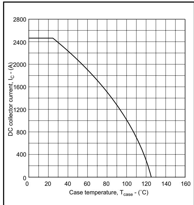
Fig. 12 DC current rating vs case temperature
