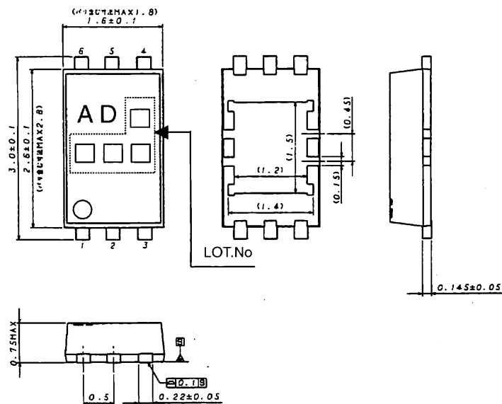
HVSO6-6 (Unit:mm)
