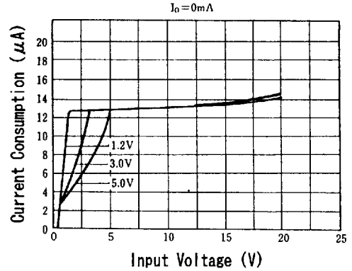
Current Consumption vs. Input Voltage
