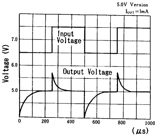
Input Transient Response
