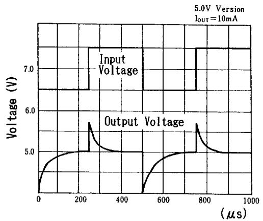
Input Transient Response
