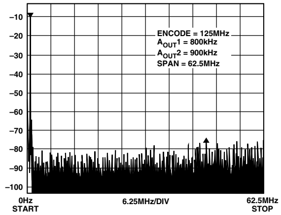
TPC 17. Wideband Intermodulation Distortion F1 = 800 \text{ kHz} ; F2 = 900 \text{ kHz} ; 125 MHz Clock; Span = 62.5 MHz
