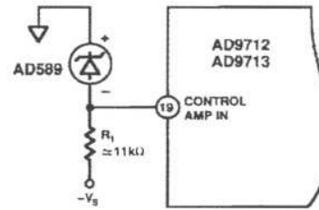
Figure 1. Use of AD589 as External Reference
