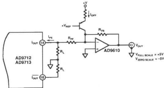
Figure 5. I/V Conversion Using Current Feedback Amp
