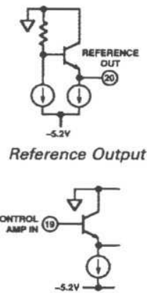
Reference Output
