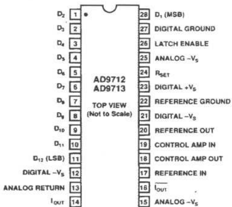
Plastic DIP Pinout Designations (Top View)
