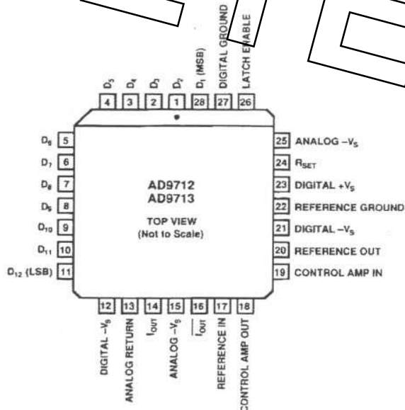
PLCC Pinout Designations
