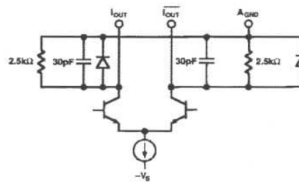
Output Circuit
