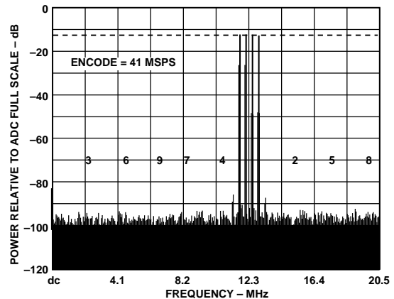
Figure 56. Multitone Performance
