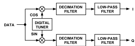
Figure 51. Digital Channelizer
