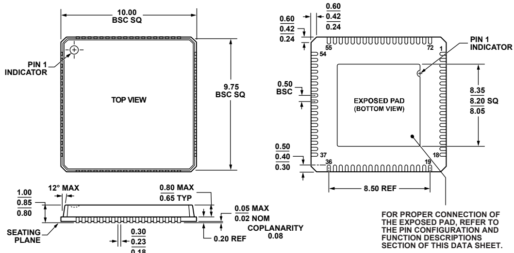
Figure 65. 72-Lead Lead Frame Chip Scale Package [LFCSP_VQ] 10 mm × 10 mm Body, Very Thin Quad (CP-72-3) Dimensions shown in millimeters
