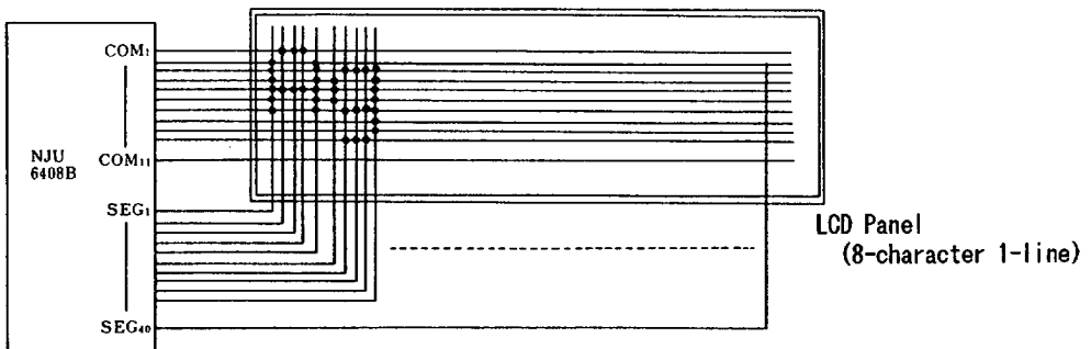
(b) 5x10 Dot 8-character 1-line example (1/4 bias, 1/11 duty)
