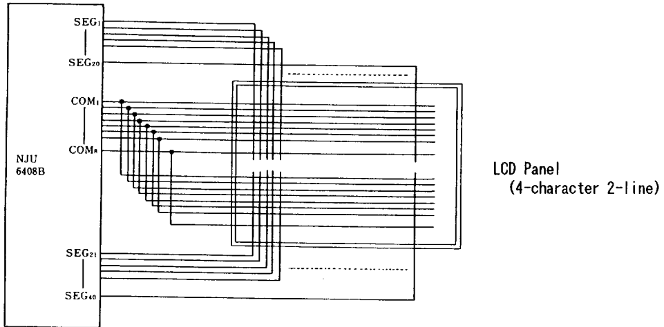
(b) 5x7 4-character 2-line example (1/4 bias, 1/8 duty)
