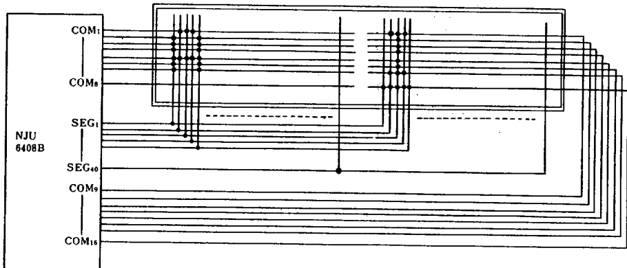
(a) 5x7 16-character 1-line example (1/5 bias, 1/16 duty)
