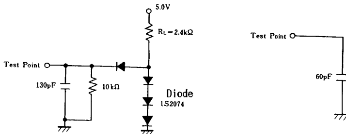
Segment extension signal load circuit
