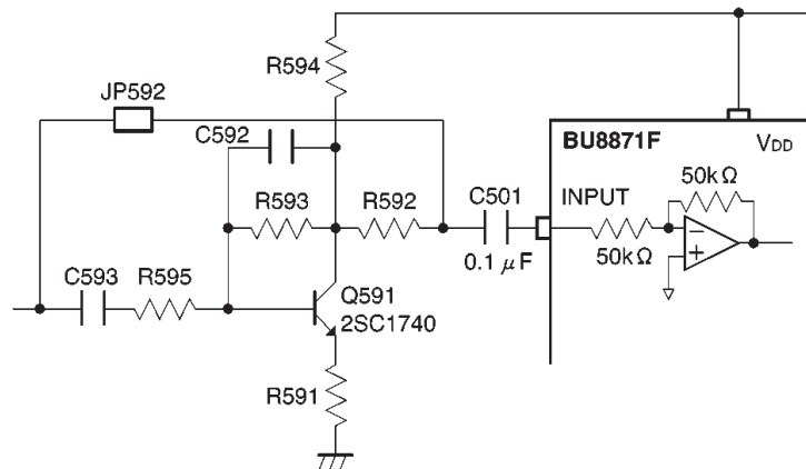
Fig. 8 DTMF input circuit
