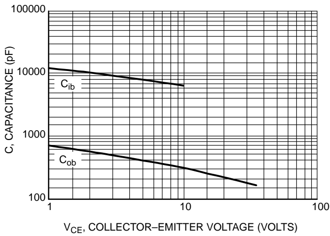
Figure 7. Typical Capacitance
