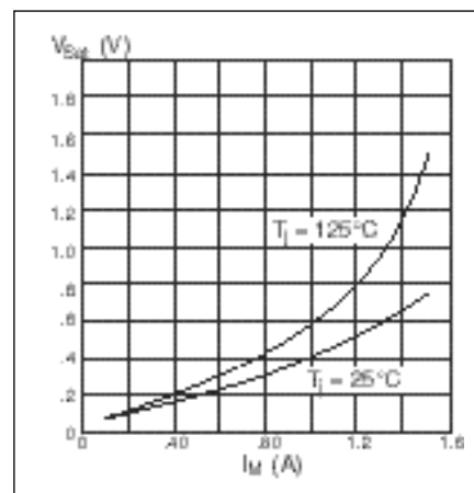
Figure 13. Typical sink saturation vs. output current
