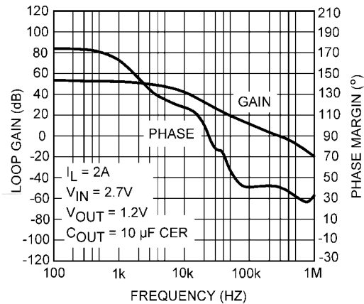
FIGURE 2. Gain-Bandwidth Plot for 2A Load
