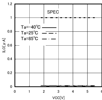
Fig.11 Output leak current I_{LO} (DO)
