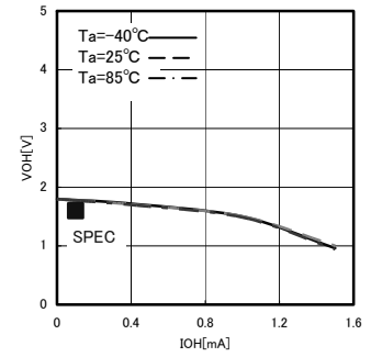
Fig.7 H output voltage V_{OH} - I_{OH} ( V_{CC}=1.8\text{V} )
