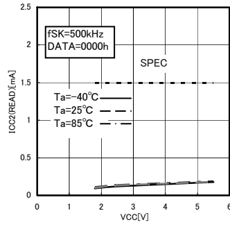
Fig.15 Consumption current at READ action ICC2 (READ, fSK=500kHz)
