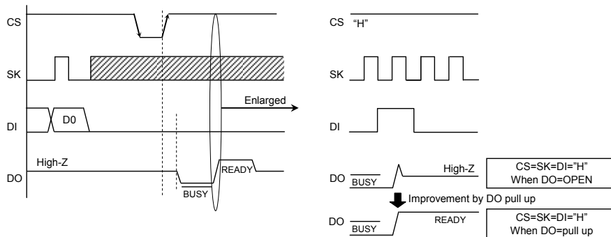
Fig.45 READY output timing at DO=OPEN
