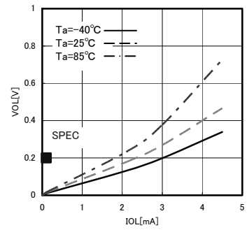
Fig.4 L output voltage V_{OL} - I_{OL} ( V_{CC}=1.8\text{V} )
