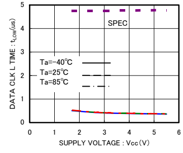
Fig.14 Data clock Low Period t_{LOW}
