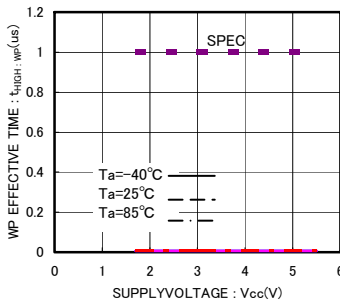
Fig.30 WP effective time t_{\text{HIGH:WP}}
