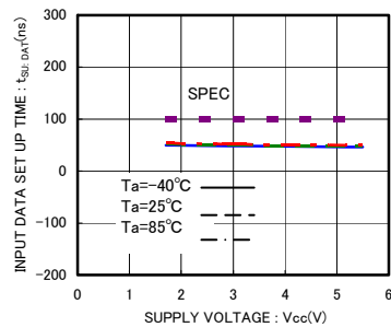
Fig.19 Input Data Setup Time t_{SU:DAT(HIGH)}
