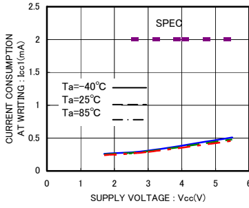
Fig.9 Current consumption at WRITE operation I_{CC1} (fsc1=400kHz)
