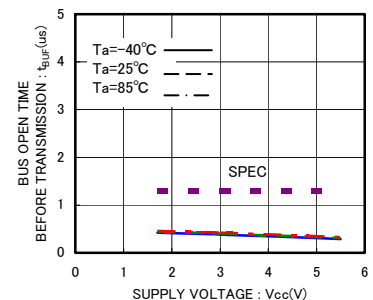
Fig.23 BUS open time before transmission t
