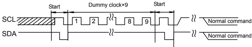
Fig.385-(b) The case of START+9 Dummy clock + START + command input
