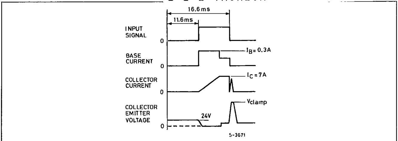
Figure 3 : Functional Test Waveforms.
