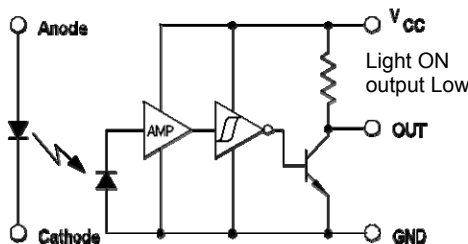
OPB916BOC Open-Collector
