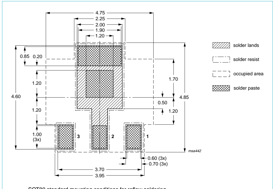
SOT89 standard mounting conditions for reflow soldering Dimensions in mm
