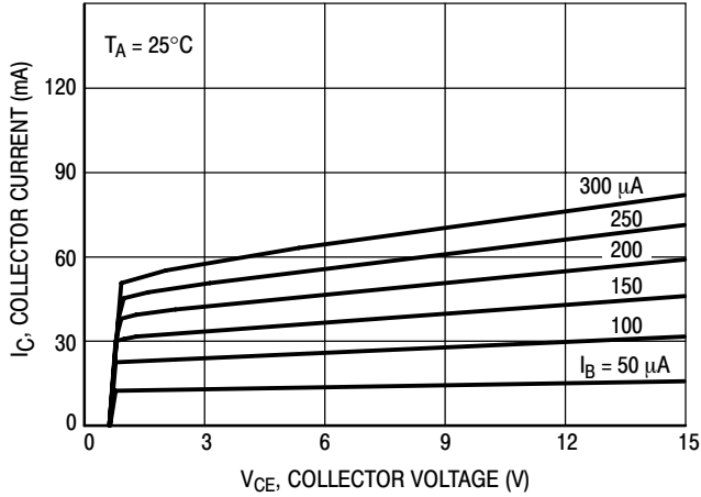
Figure 1. I_C - V_{CE}
