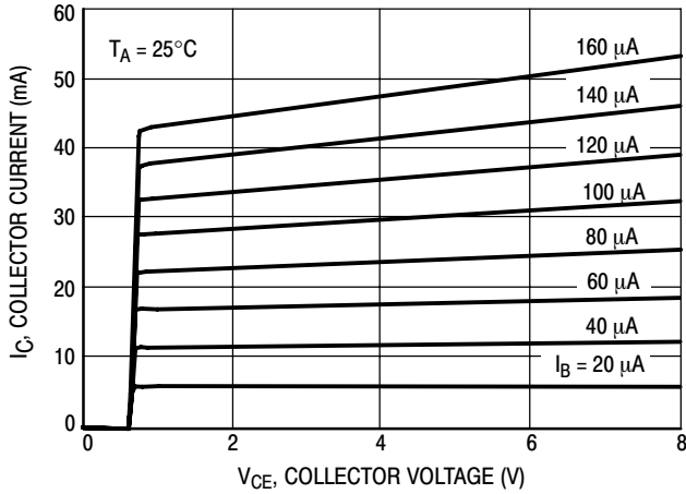
Figure 1. I_C - V_{CE}
