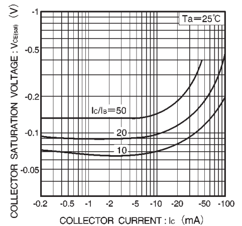
Fig.17 Collector-emitter saturation voltage vs. collector current (I)
