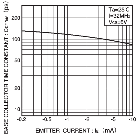
Fig.11 Base-collector time constant vs. emitter current
