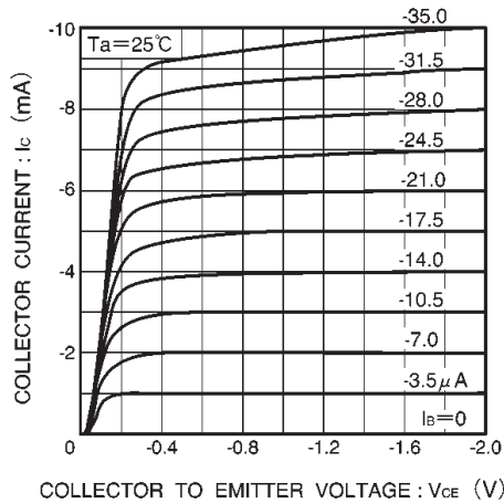
Fig.13 Grounded emitter output characteristics (I)
