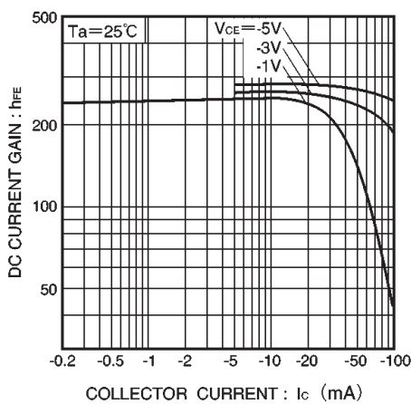
Fig.15 DC current gain vs. collector current (I)
