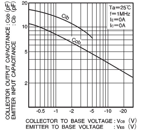
Fig.20 Collector output capacitance vs. collector-base voltage Emitter input capacitance vs. emitter-base voltage
