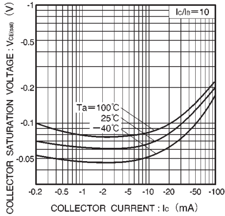
Fig.18 Collector-emitter saturation voltage vs. collector current ( I )
