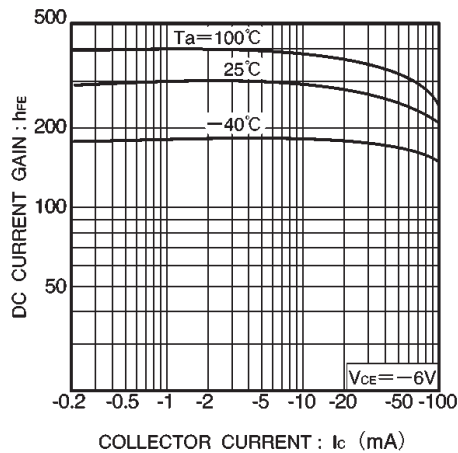
Fig.16 DC current gain vs. collector current (II)
