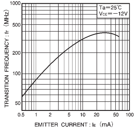
Fig.19 Gain bandwidth product vs. emitter current
