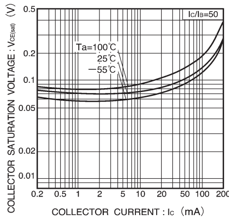
Fig.8 Collector-emitter saturation voltage vs. collector current (III)
