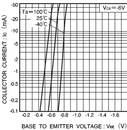
Fig.12 Grounded emitter propagation characteristics
