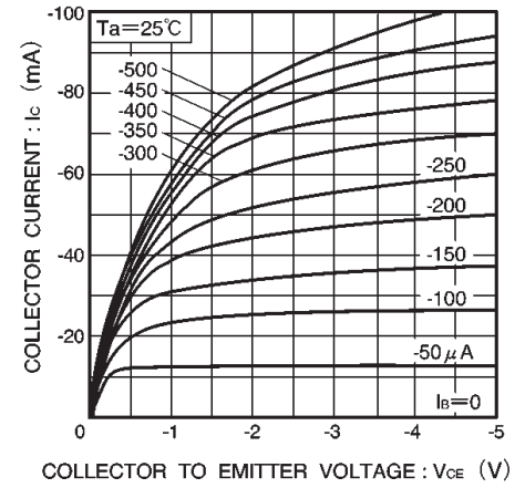
Fig.14 Grounded emitter output characteristics (II)
