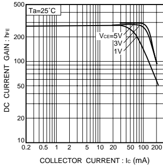
Fig.13 DC current gain vs. collector current ( I )
