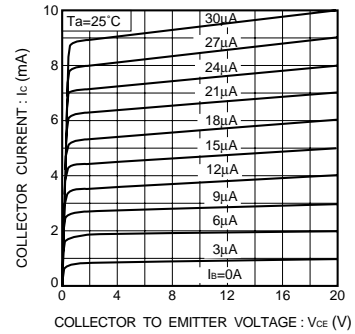
Fig.12 Grounded emitter output characteristics ( II )
