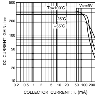
Fig.14 DC current gain vs. collector current ( II )
