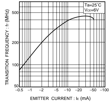
Fig.18 Gain bandwidth product vs. emitter current
