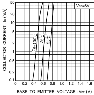
Fig.10 Grounded emitter propagation characteristics
