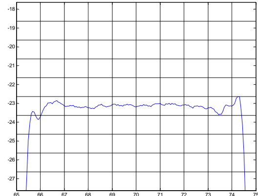
Phase Linearity( f_0 \pm 4\text{MHz} )
