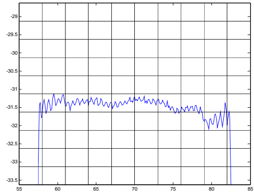
Phase Linearity(f0±12MHz)
