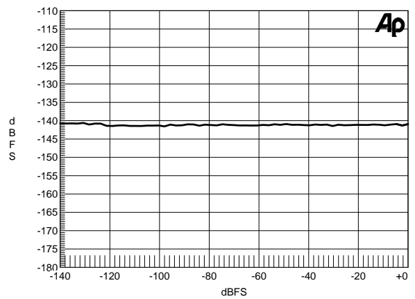
Figure 62. THD+N vs. Input Amplitude, 1 kHz Tone, 192 kHz:48 kHz
