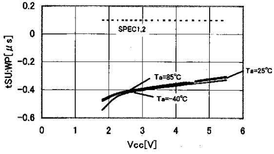
WP SETUP TIME t_{SU:WP}
