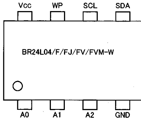
Fig.-3 PIN LAYOUT
