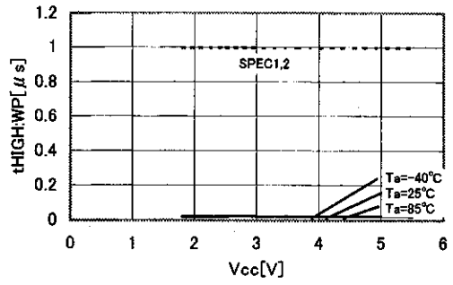
WP HIGH PERIOD t_{HIGH:WP}
