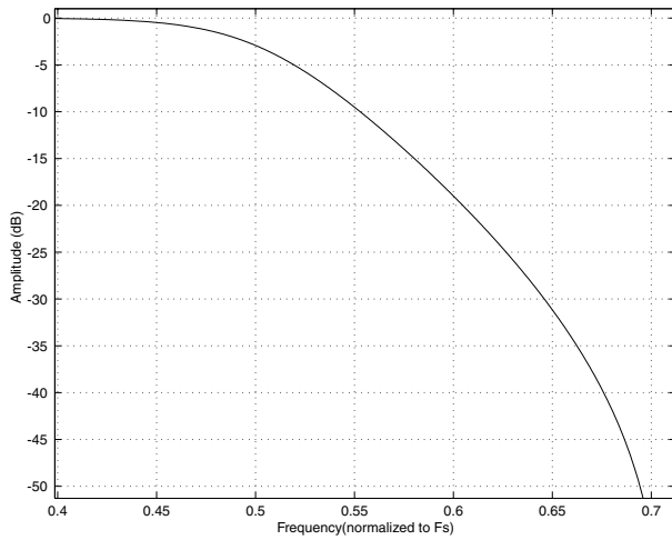
Figure 24. Quad Speed Transition Band
