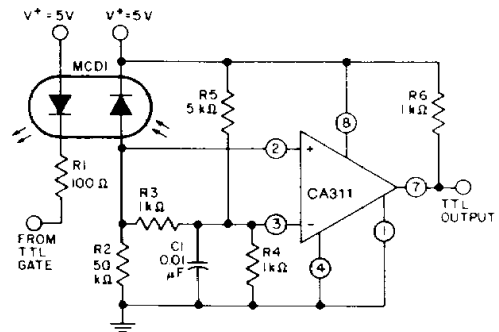
Fig. 18 - Digital transmission isolator.
