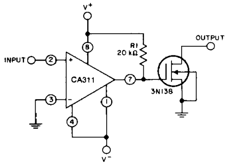
Fig. 23 - Zero-crossing detector driving and MOS switch.
