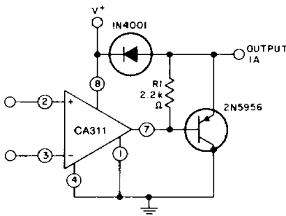
Fig. 17 - Comparator and solenoid driver.
