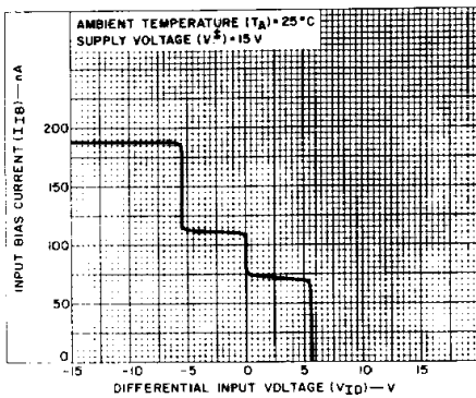
Fig. 10 - Input characteristics.
