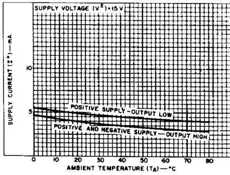
Fig. 14 - Supply current vs. ambient temperature.
