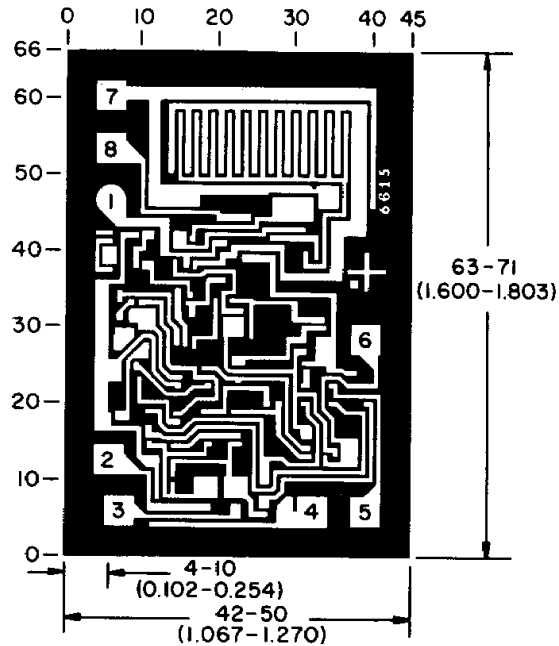
Fig. 33 - Switching power amplifier.
