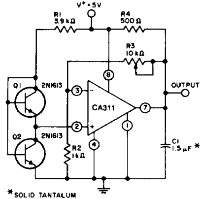
Fig. 22 - Low-voltage adjustable-reference supply.
