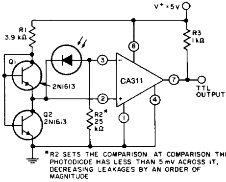
Fig. 25 - Precision photodiode comparator.
