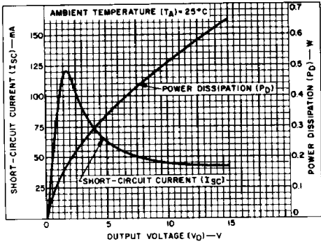
Fig. 6 - Output limiting characteristics.
