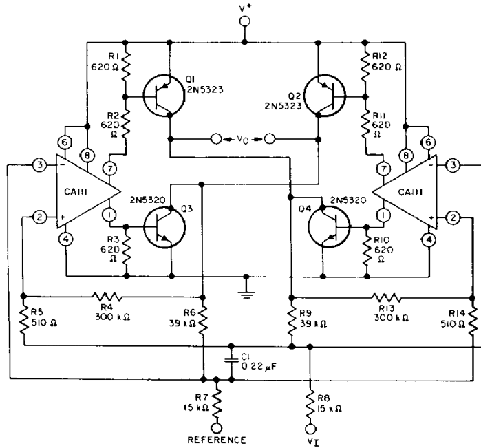
Fig. 33 - Switching power amplifier.
