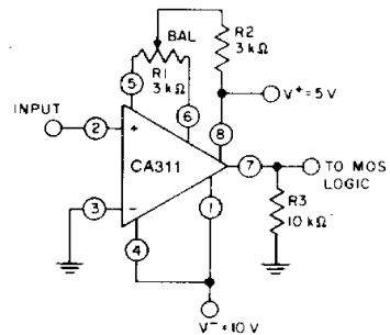
Fig. 20 - Zero-crossing detector driving MOS logic.
