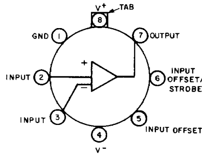
FUNCTIONAL DIAGRAM FOR TO-5 STYLE PACKAGE.
