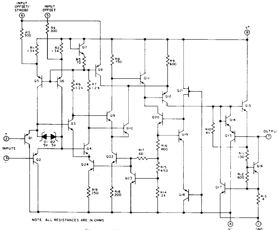
Figure 1 - Schematic diagram of CA311.
