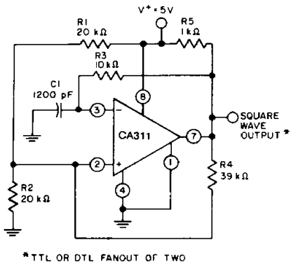
Fig. 26 - 100-kHz free-running multivibrator.
