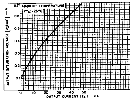
Fig. 13 - Output saturation voltage vs. output current.
