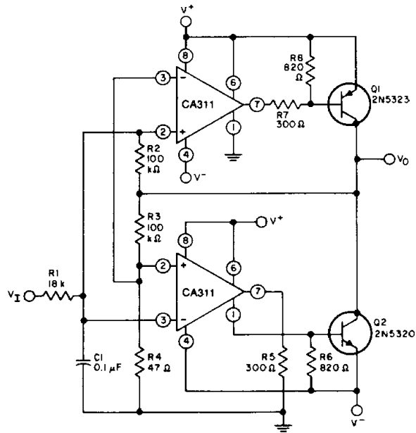
Fig. 27 - Switching power amplifier.
