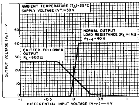
Fig. 12 - Transfer function.
