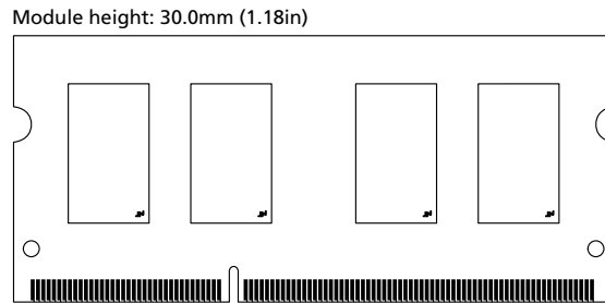
Figure 1: 204-Pin SODIMM (MO-268 R/C B)
