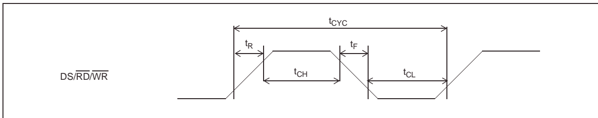
Figure 18 - \overline{DS}/\overline{RD}/\overline{WR} Clock Pulse
