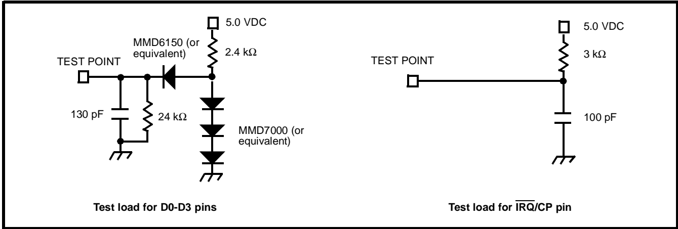
Figure 14 - Test Circuits
