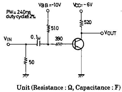
t_{stg} Test Circuit
