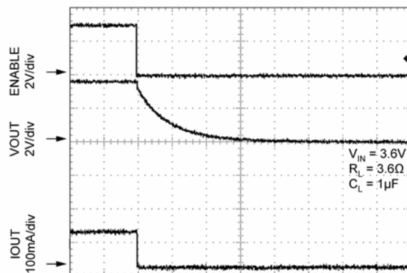
Turn-On/Turn-Off Timing
