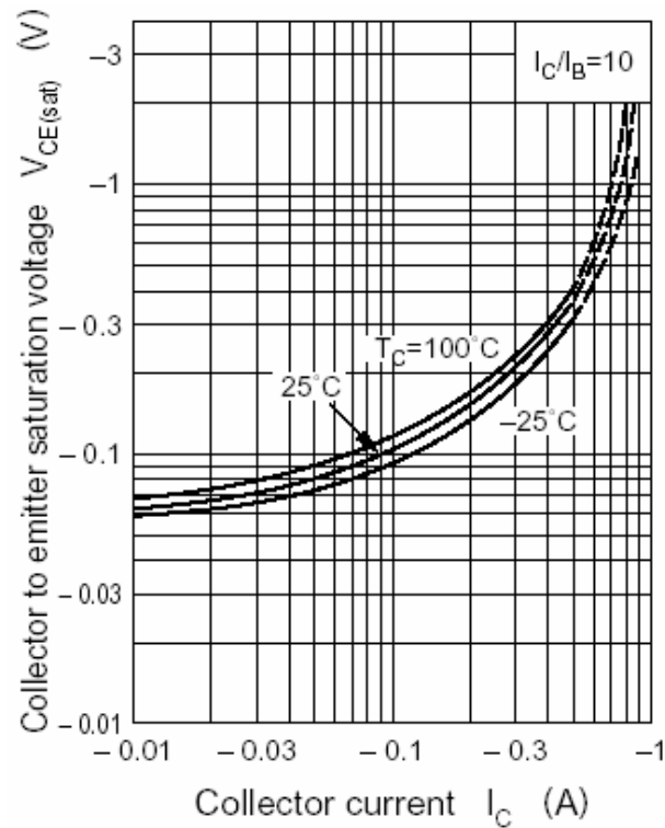
Fig.3 Collector-Emitter Saturation Voltage
