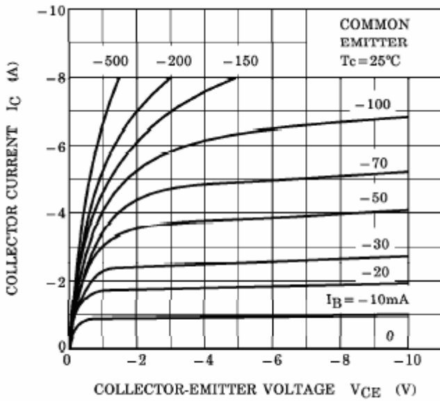
Fig.3 Static Characteristic
