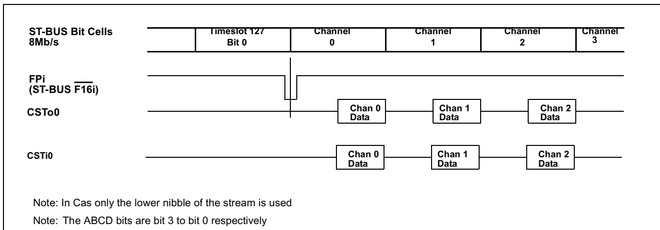
Figure 60 - ST-BUS 8.192Mb/s Functional Timing Diagram for CSTo/CSTi CAS
