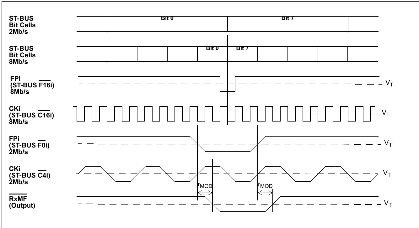
Figure 66 - Receive Multiframe (CRC-4 or CAS) Timing
