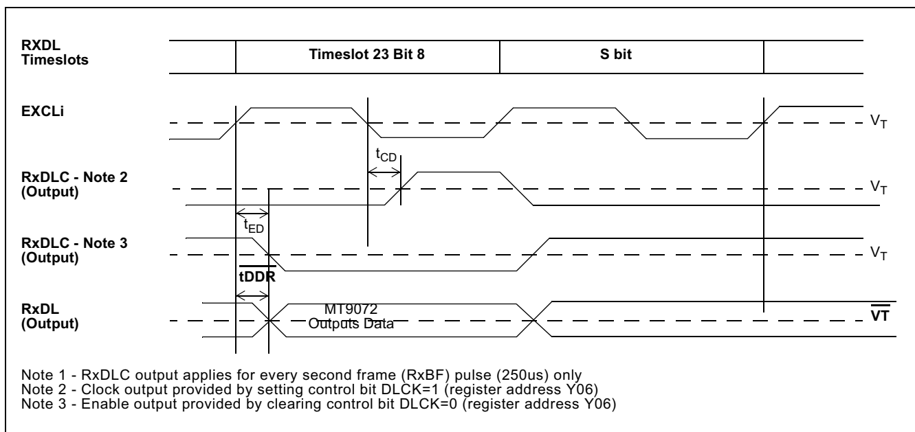
Figure 43 - Receive DataLink Timing Diagram
