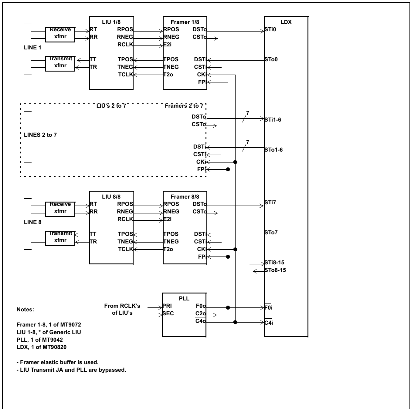
Figure 20 - 8 E1 Links with no JA or PLL in LIU, Slave or Master Mode, Jitter-Free ST-BUS
