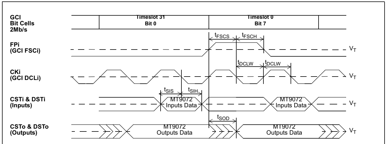
Figure 28 - GCI 2.048 Mb/s Timing Diagram
