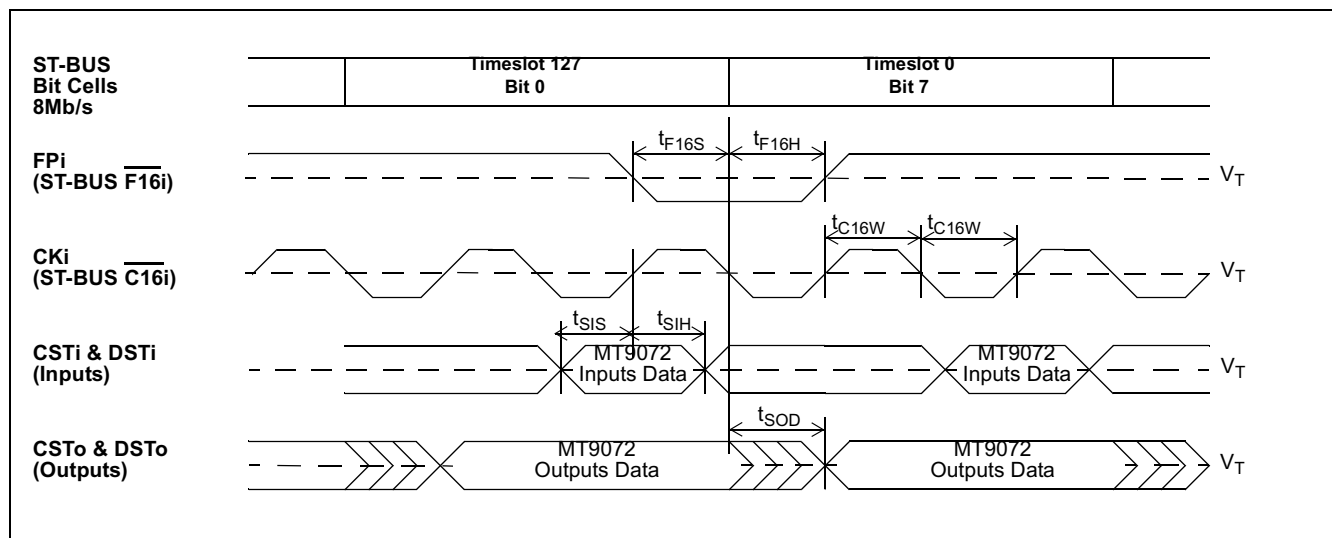
Figure 58 - ST-BUS 8.192Mb/s Timing
