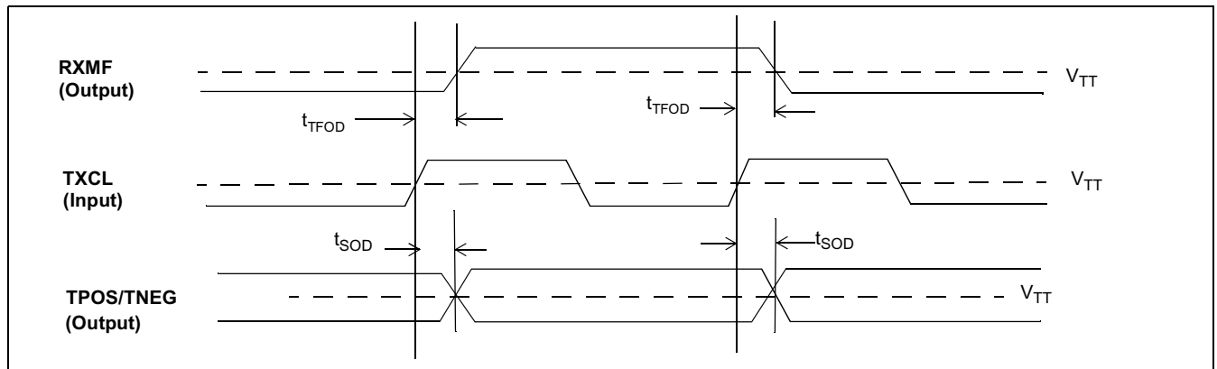
Figure 40 - Receive Multiframe Timing with TX8KE n Set Timing Diagram
