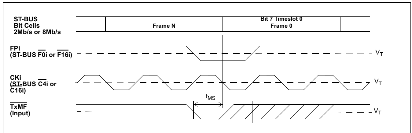
Figure 64 - Transmit Multiframe (CRC-4 or CAS) Timing
