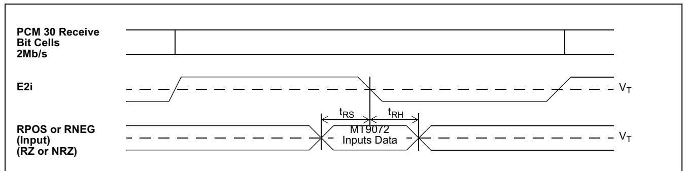
Figure 77 - PCM 30 Receive Timing
