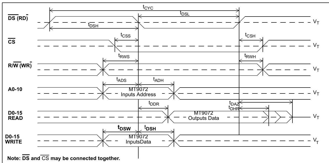
Figure 25 - Motorola Microprocessor Timing
