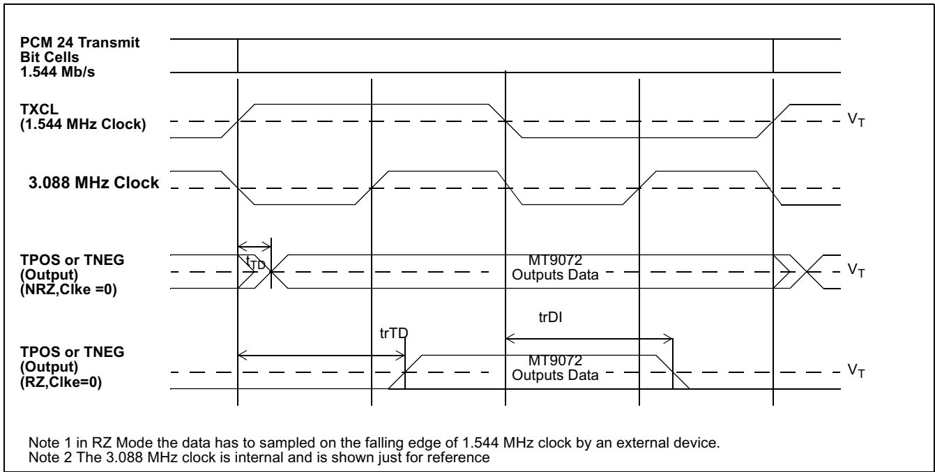
Figure 45 - PCM 24 Transmit Timing
