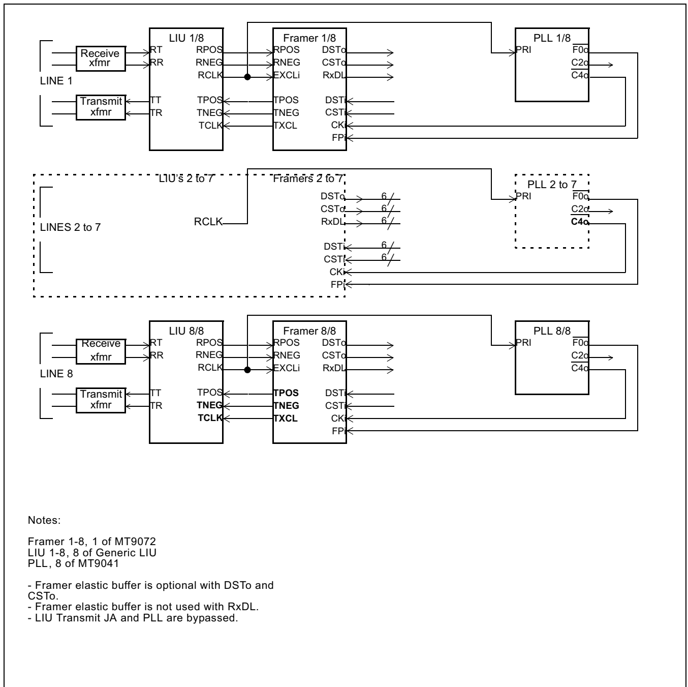
Figure 14 - 8 T1 Links with Asynchronous ST-BUS
