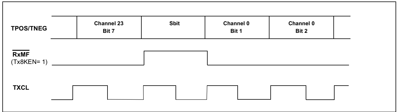
Figure 39 - Receive Multiframe Timing with TX8KE n Set Functional Timing Diagram
