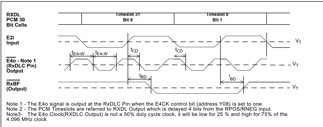
Figure 72 - Receive Basic Frame and E4o Timing
