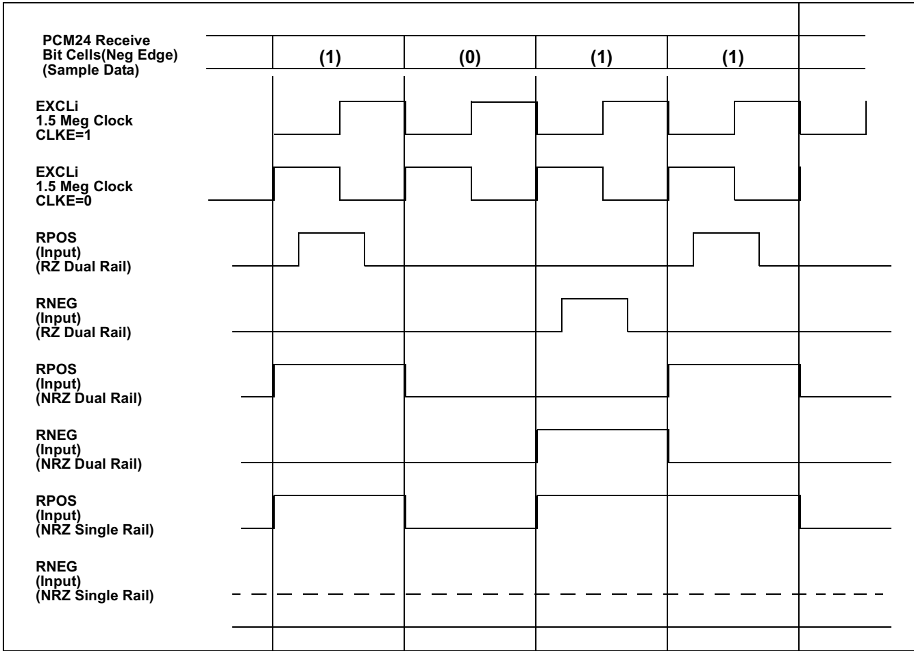
Figure 47 - PCM24 Receive Functional Timing
