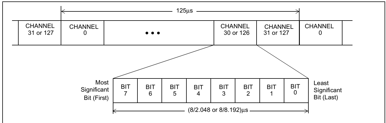
Figure 80 - ST-BUS Format
