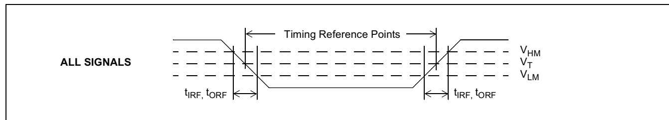
Figure 51 - Timing Parameter Measurement Voltage Levels
