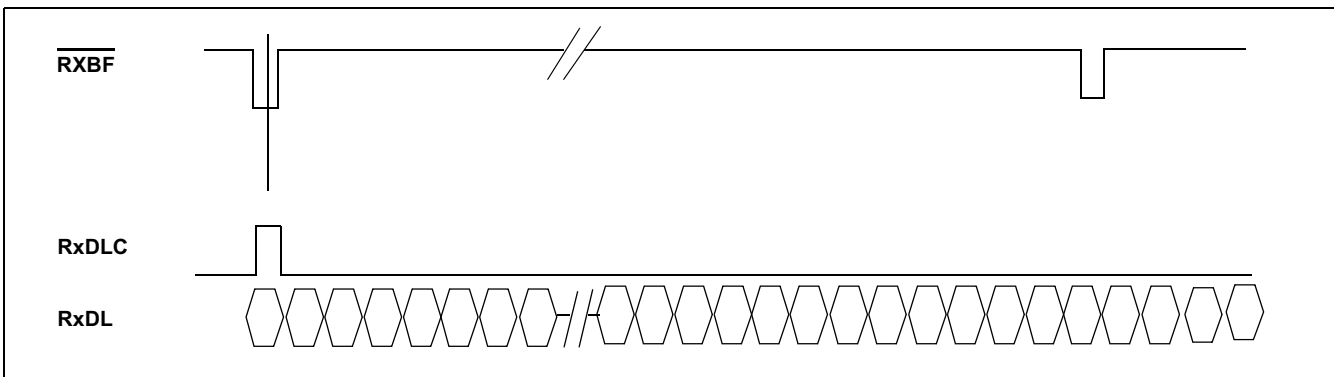
Figure 42 - Receive Data Link Functional Diagram
