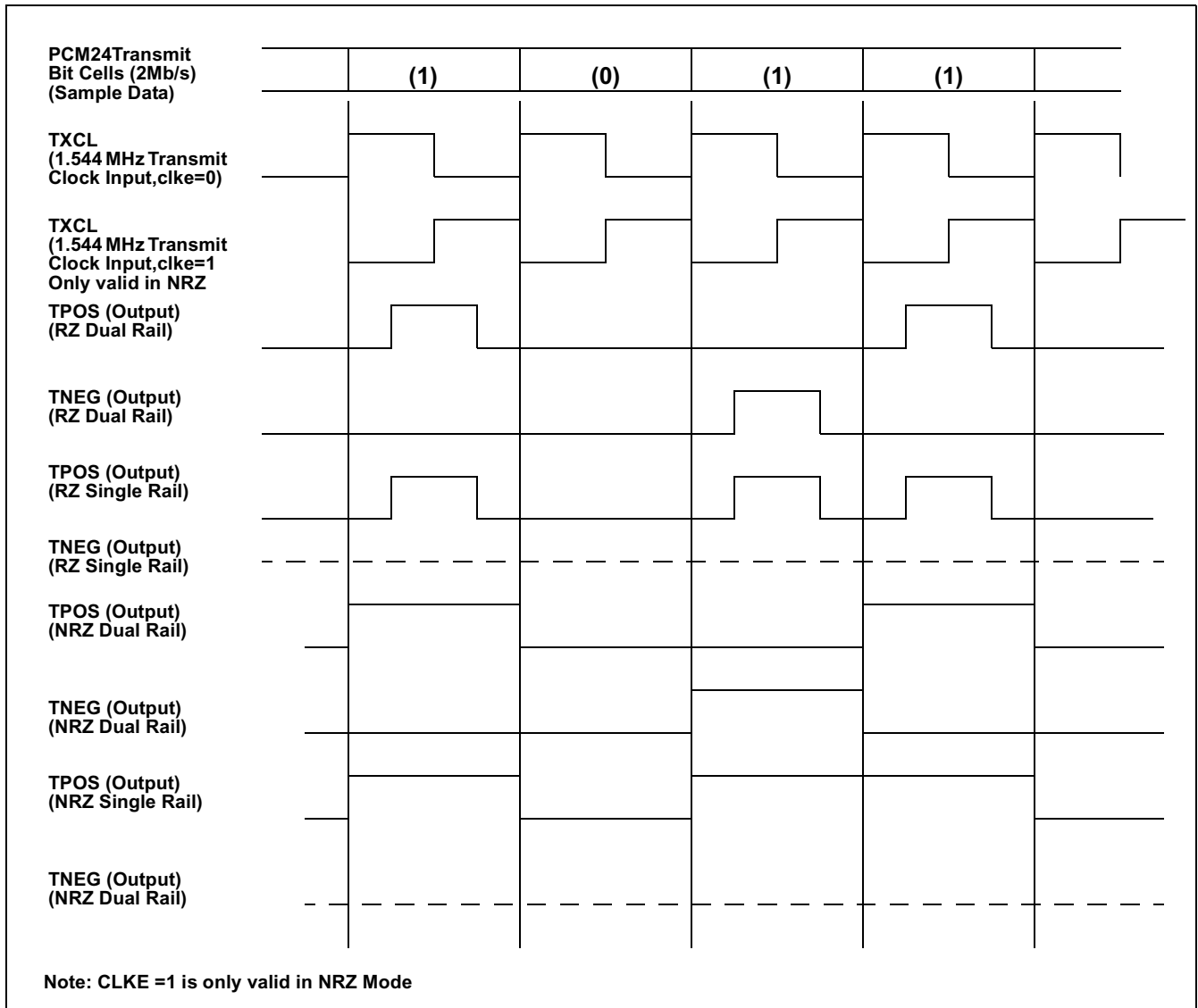
Figure 46 - PCM24 Transmit Functional Timing
