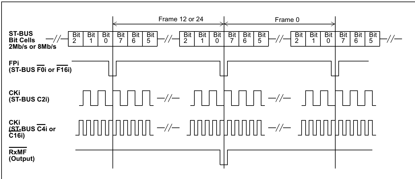
Figure 37 - Receive Multiframe Functional Timing
