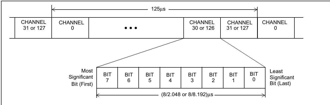
Figure 5 - ST-BUS Format
