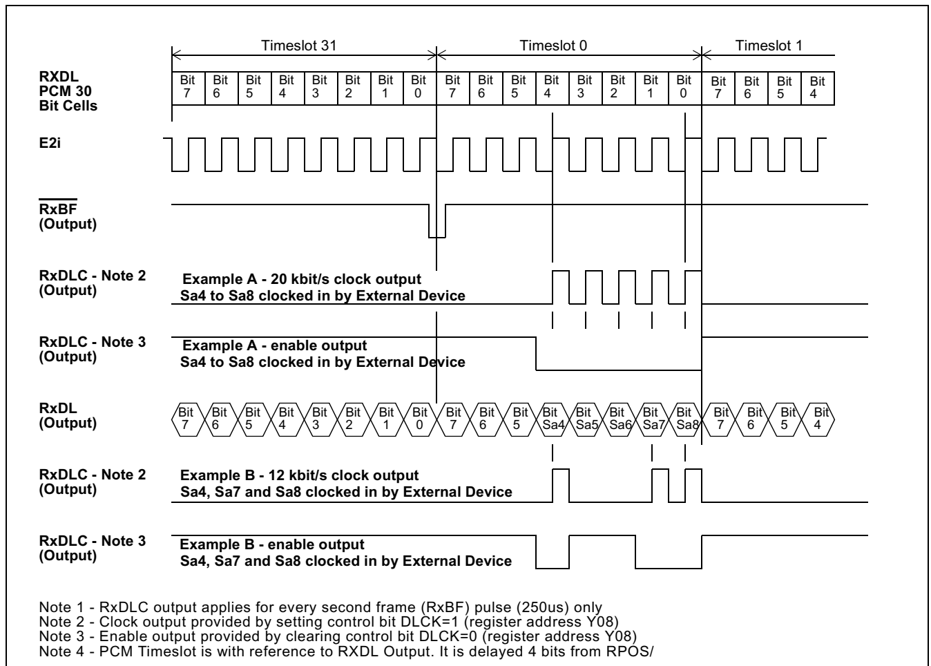
Figure 74 - Receive Data Link Pin Functional Timing
