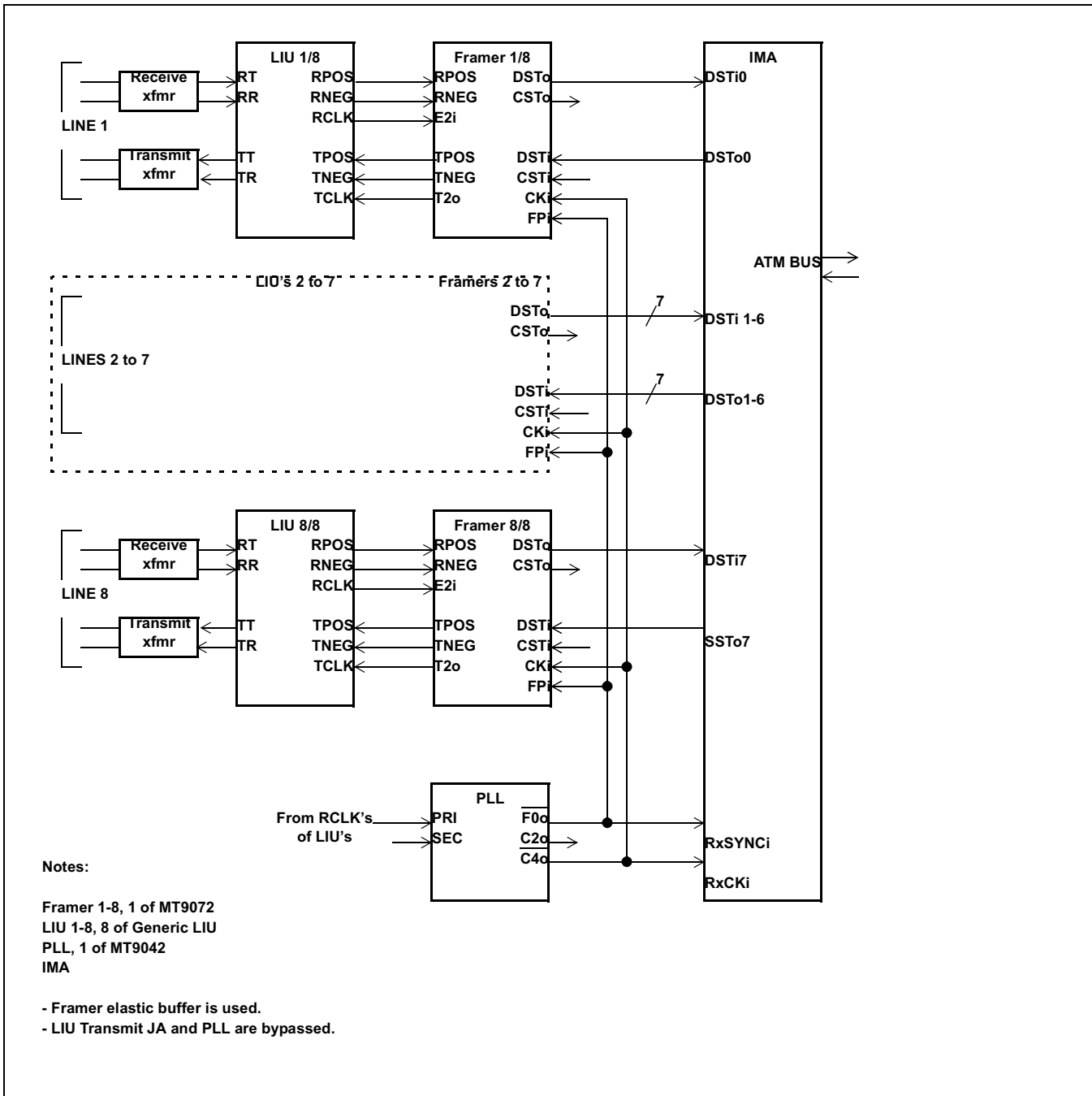
Figure 21 - 8 E1 Links with ATM IMA with Synchronous ST-BUS Mode
