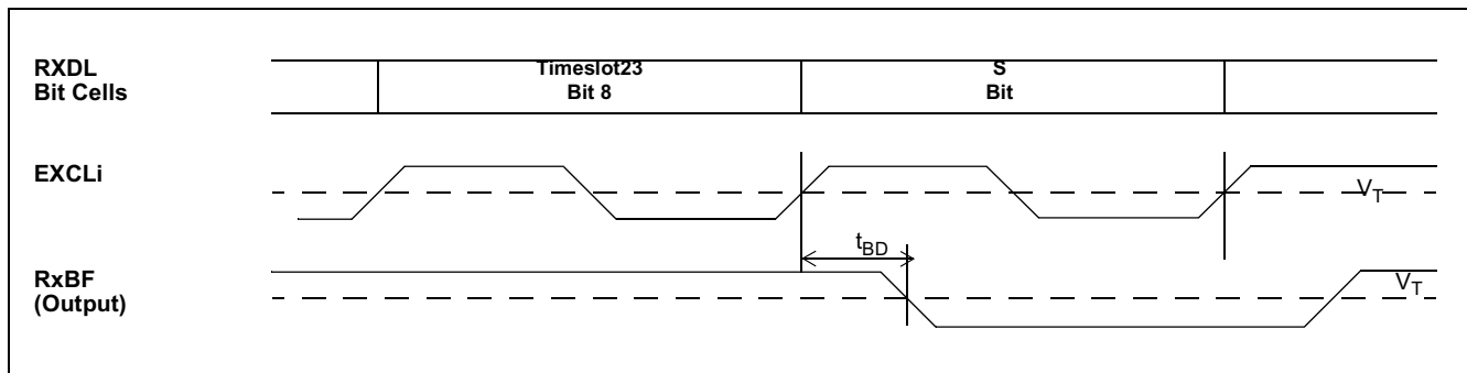
Figure 44 - Receive Basic Frame Pulse Pin Timing
