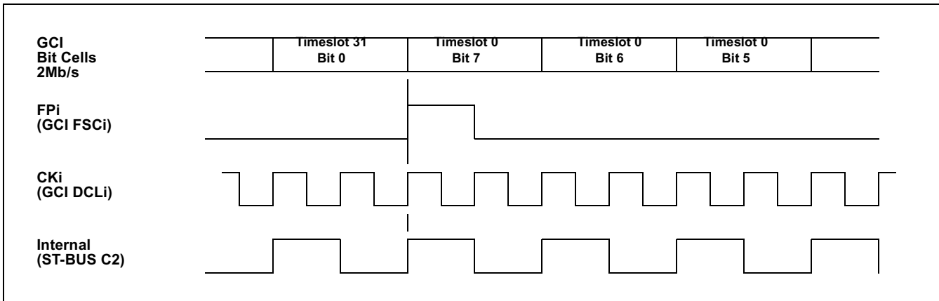
Figure 57 - GCI 2.048Mb/s Functional Timing Diagram
