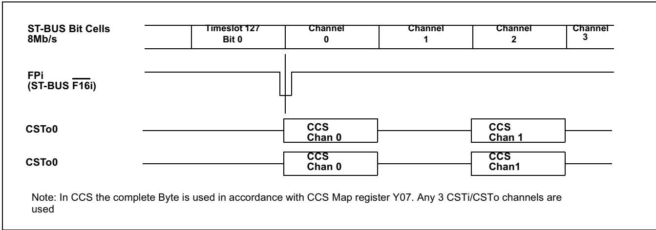
Figure 61 - ST-BUS 8.192Mb/s Functional Timing Diagram for CSTo/CSTi CAS
