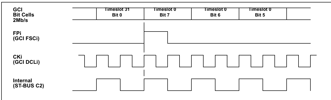
Figure 27 - GCI 2.048Mb/s Fractional Timing Diagram
