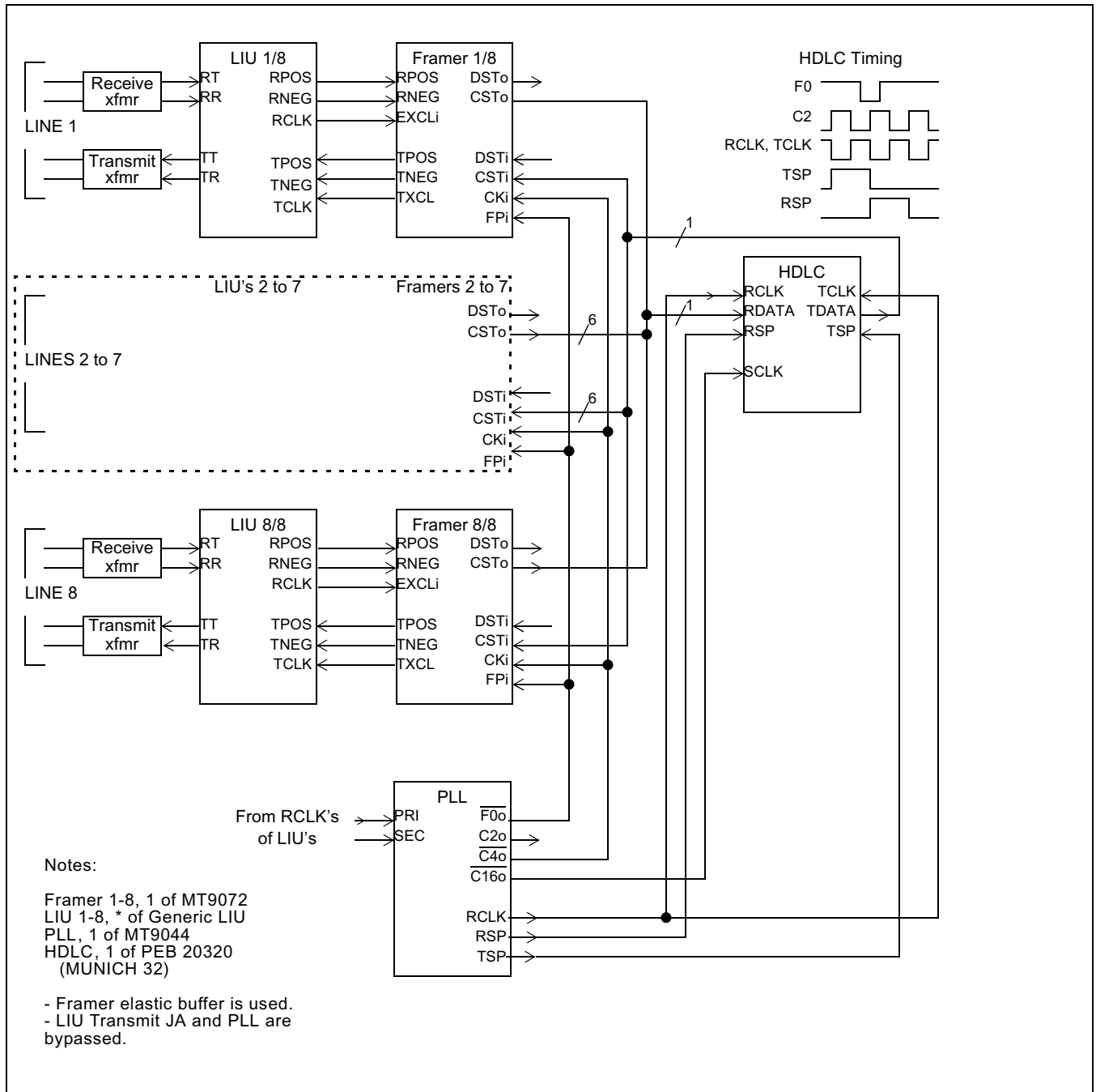
Figure 8 - 8 T1 Links with Synchronous Common Channel Signaling for up to 24 Channels
