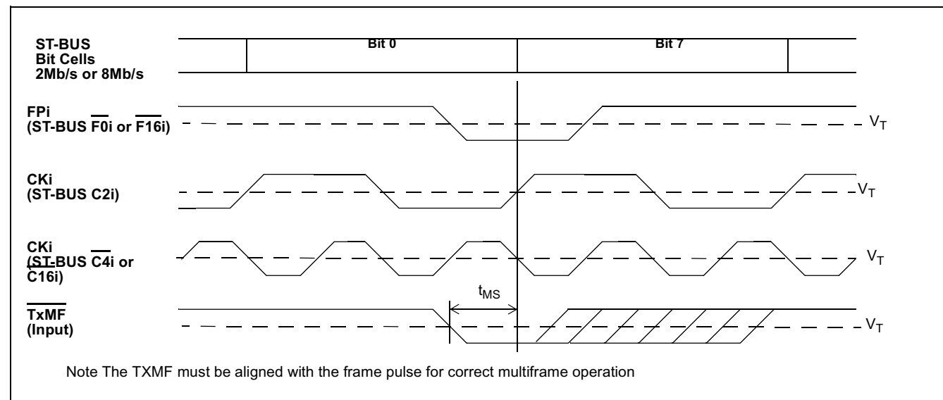
Figure 36 - Transmit Multiframe Timing
