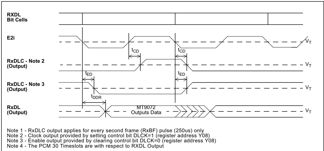
Figure 73 - Receive Data Link Timing
