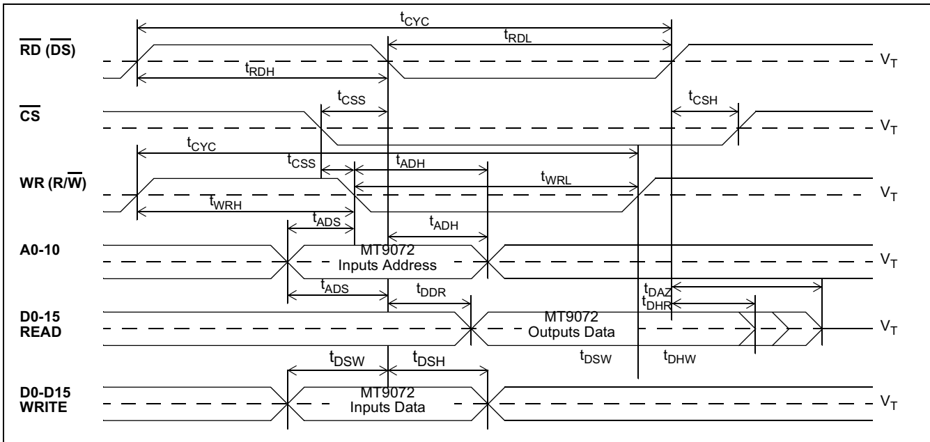
Figure 26 - Intel Microprocessor Timing
