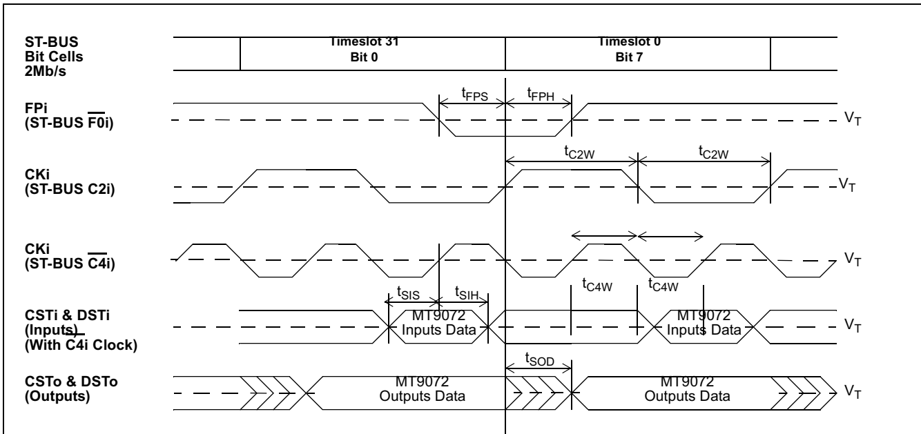
Figure 30 - ST-BUS 2.048Mb/s Timing
