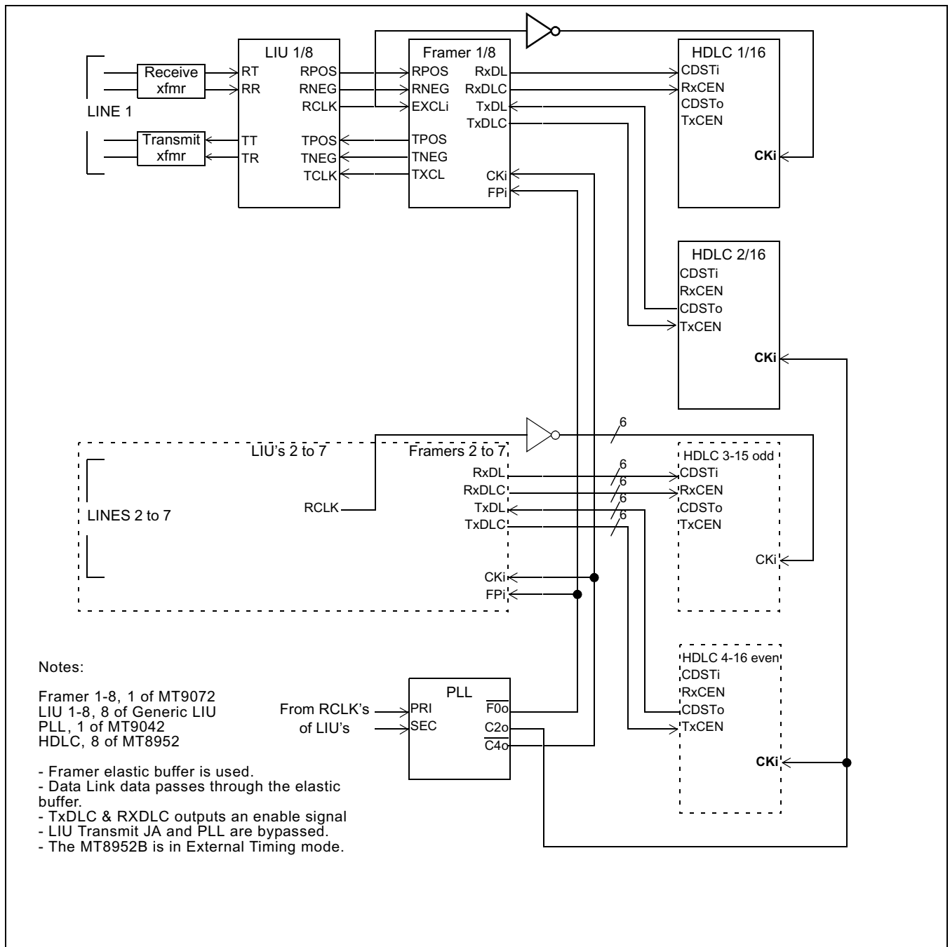
Figure 10 - 8 T1 Links with Asynchronous Data Link Signaling
