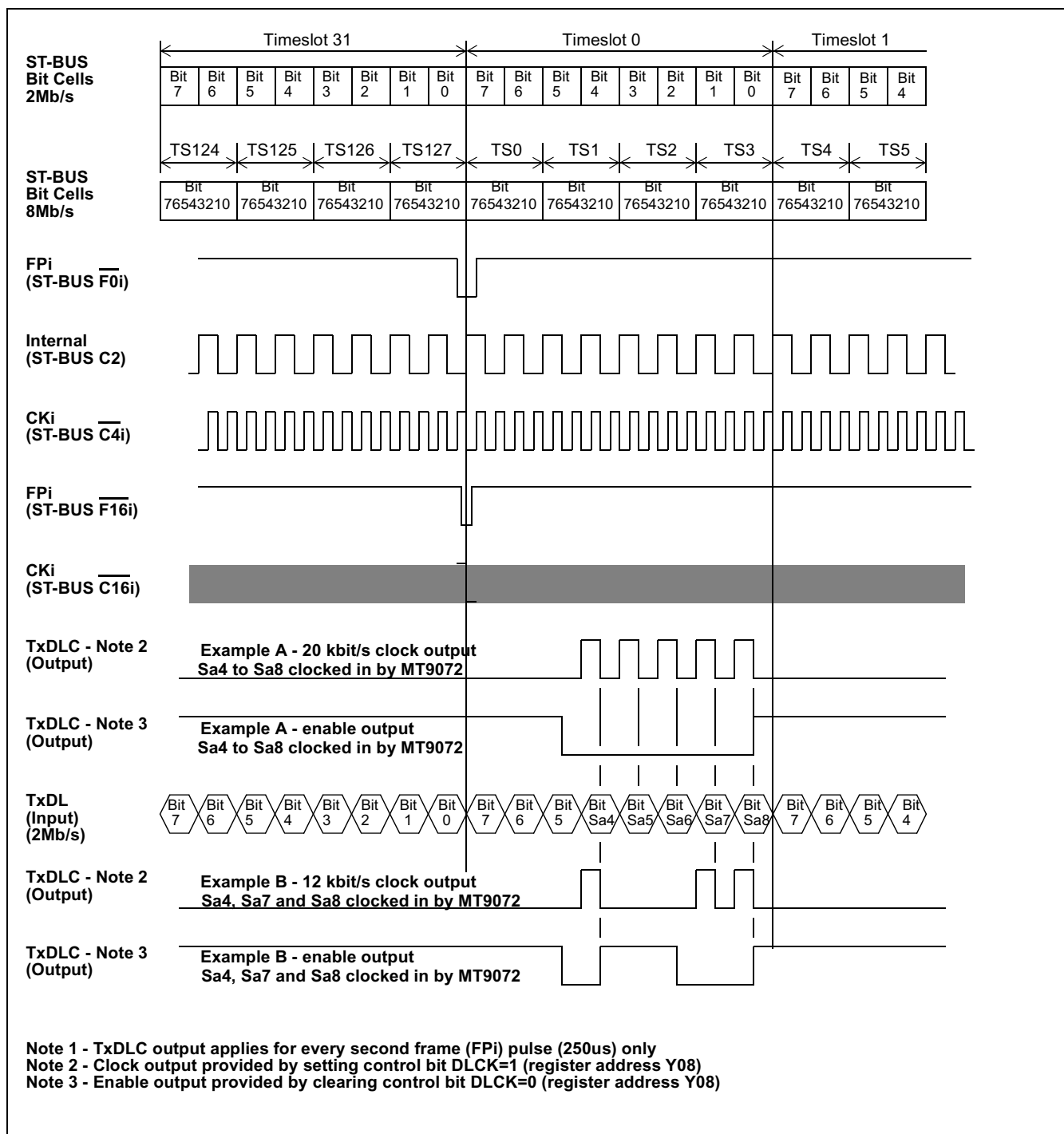
Figure 71 - Transmit Data Link Pin Functional Timing
