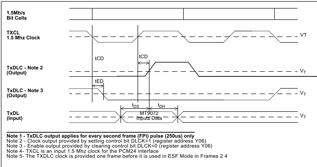
Figure 41 - Transmit Data Link Pin Timing
