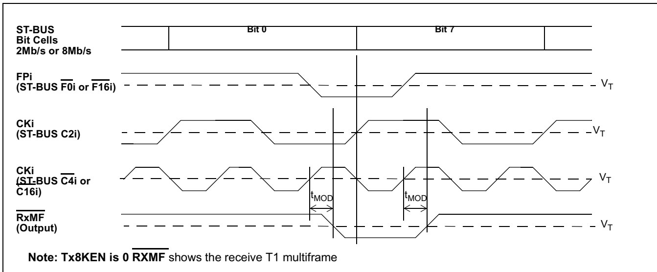
Figure 38 - Receive Multiframe Timing
