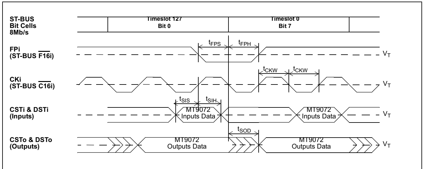
Figure 32 - ST-BUS 8.192Mb/s Timing
