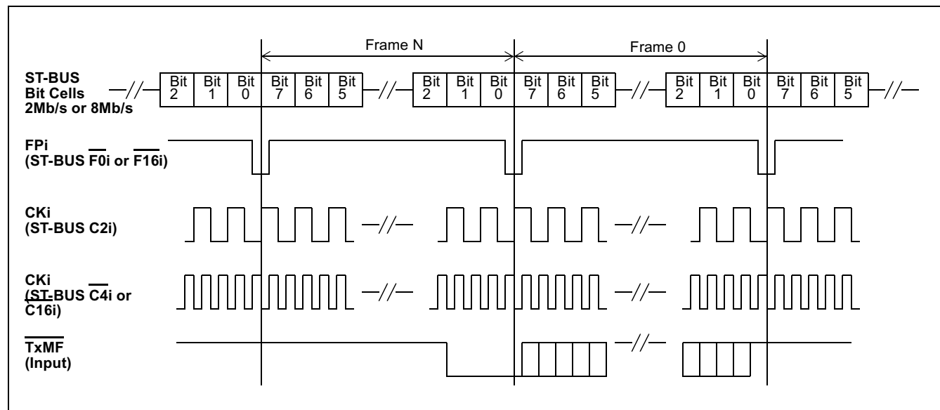
Figure 35 - Transmit Multiframe Functional Timing
