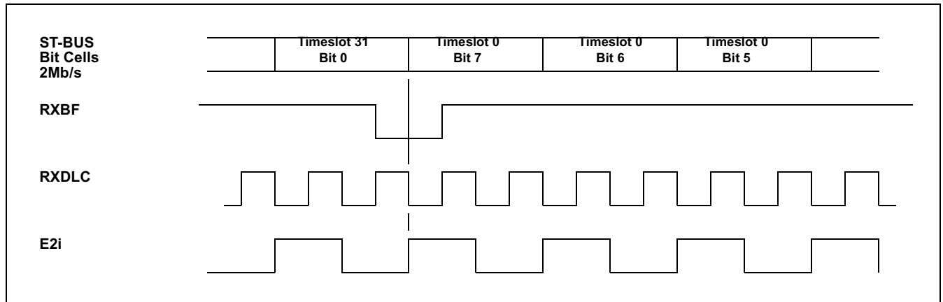
Figure 63 - Receive IMA Functional Timing Diagram
