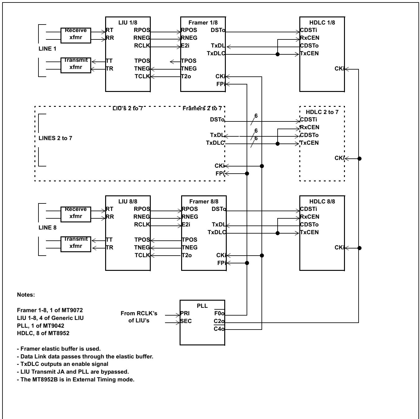
Figure 18 - 8 E1 Links with Synchronous Data Link signaling
