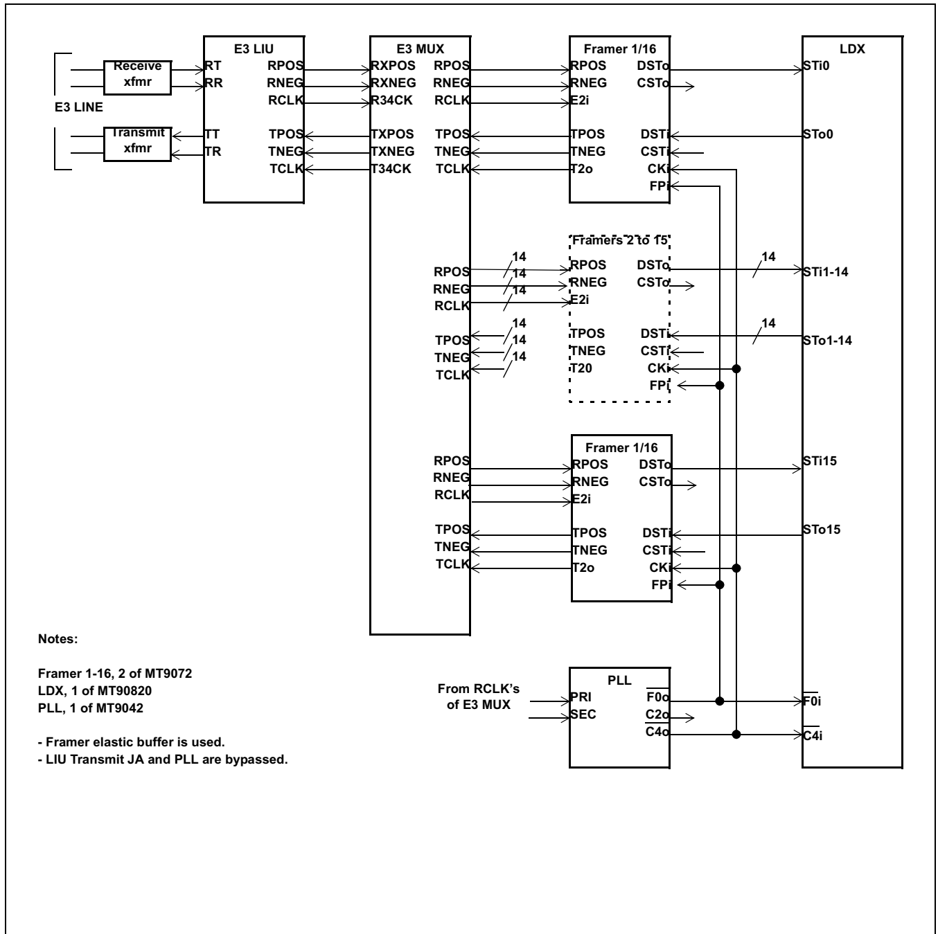
Figure 16 - E3 (34Mb/s) MUX Cross Connect with 16 Asynchronous E1 Links
