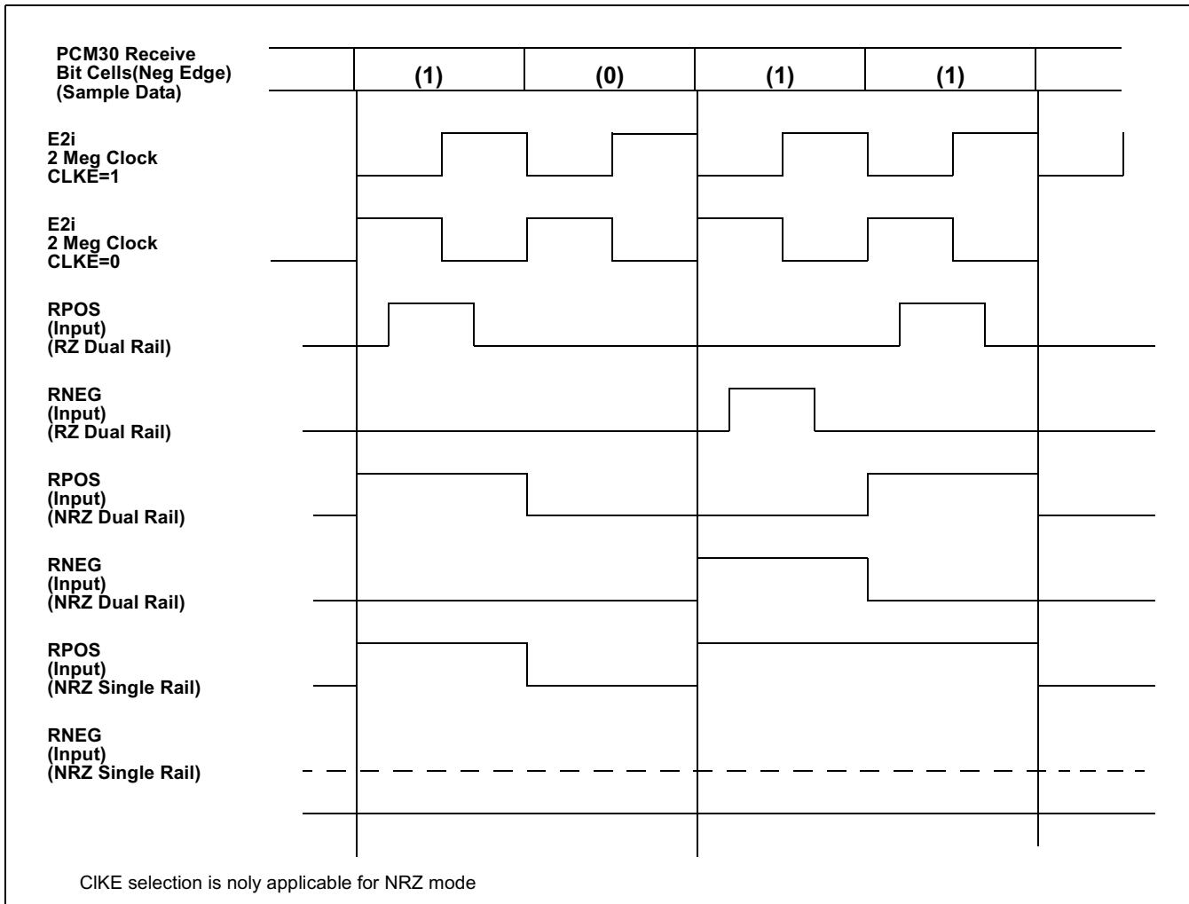
Figure 78 - PCM30 Receive Functional Timing
