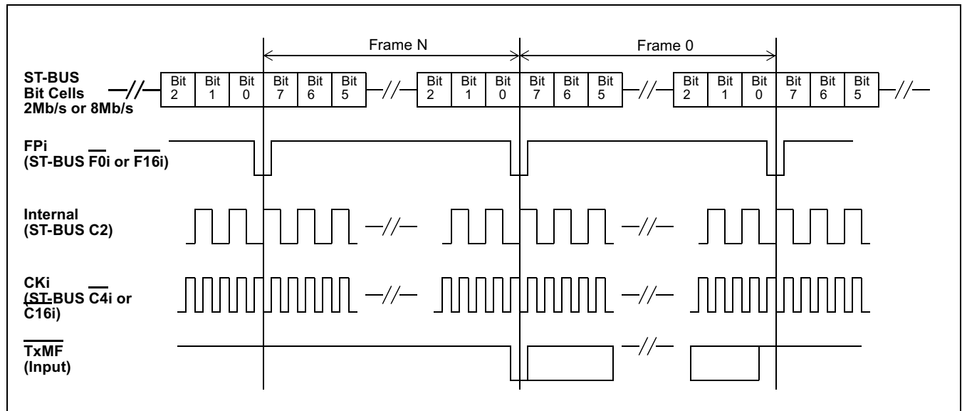
Figure 65 - Transmit Multiframe (CRC-4 or CAS) Functional Timing
