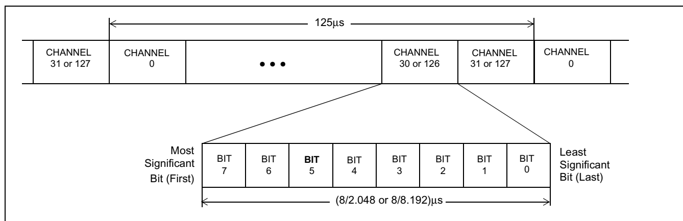
Figure 50 - ST-BUS Format
