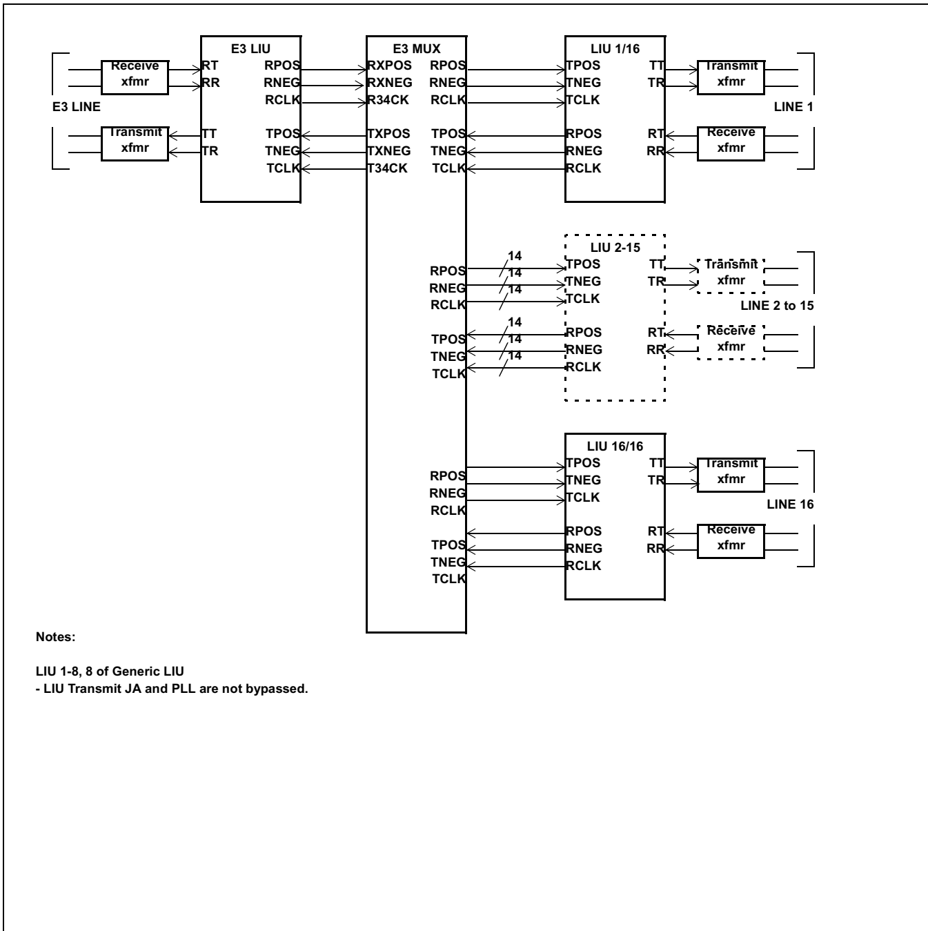
Figure 17 - E3 (34Mb/s) MUX Concentrator to 16 Asynchronous E1 Links
