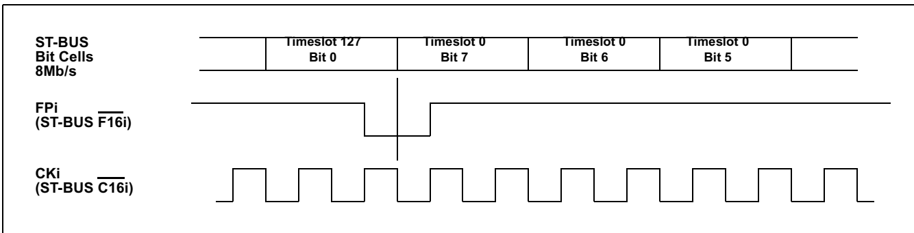
Figure 31 - ST-BUS 8.192Mb/s Functional Timing Diagram
