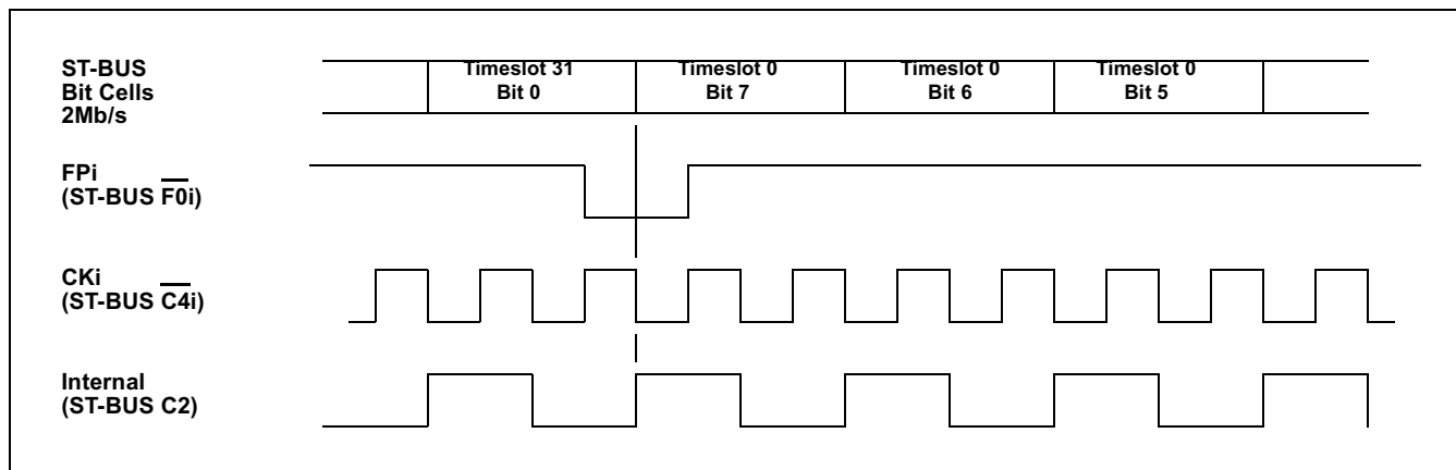
Figure 55 - ST-BUS 2.048Mb/s Functional Timing Diagram
