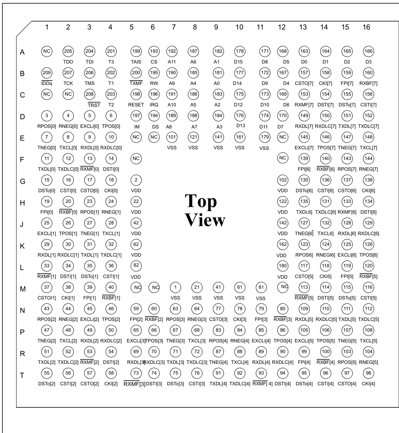
Figure 3 - 256 PIN LPGA (Jedec MO-192)
