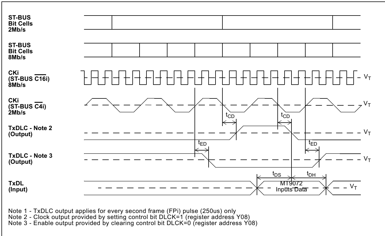
Figure 70 - Transmit Data Link Pin Timing
