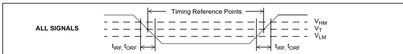
Figure 24 - Timing Parameter Measurement Voltage Levels
