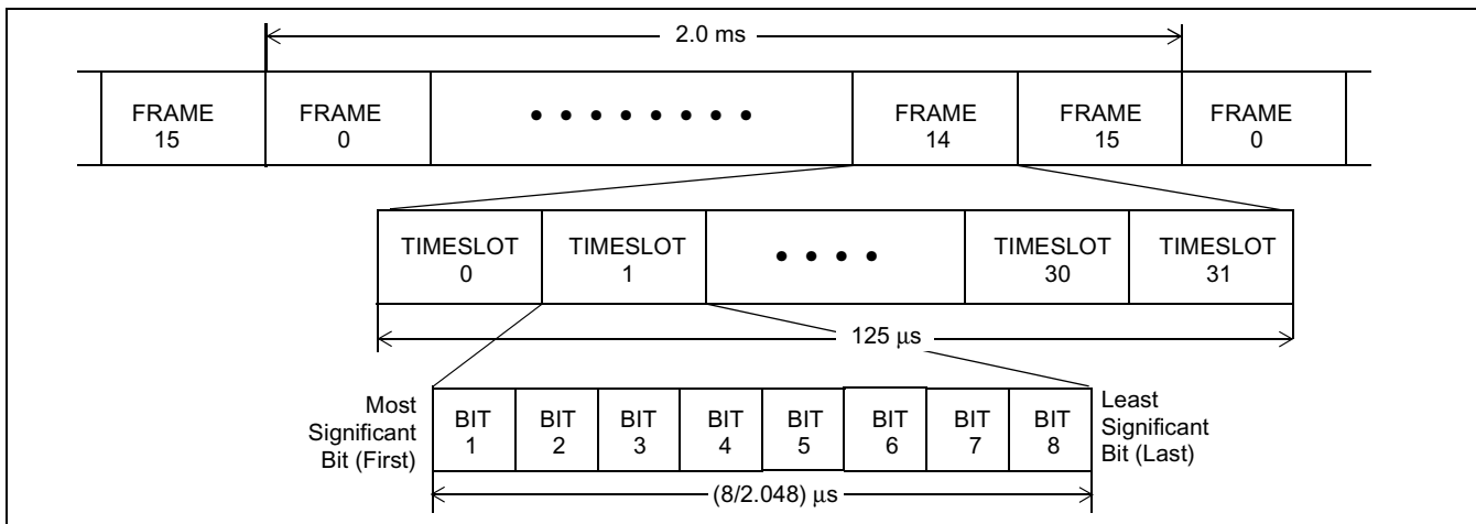
Figure 79 - PCM 30 Format
