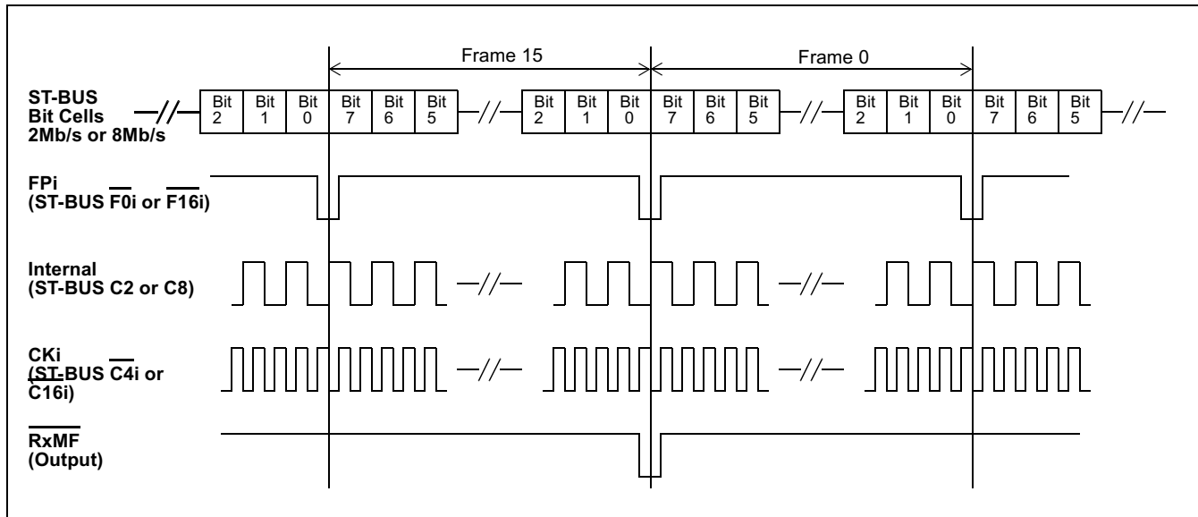
Figure 67 - Receive Multiframe (CRC-4 or CAS) Functional Timing
