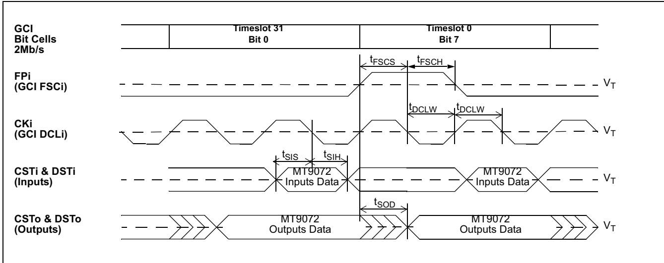
Figure 56 - GCI 2.048Mb/s Timing
