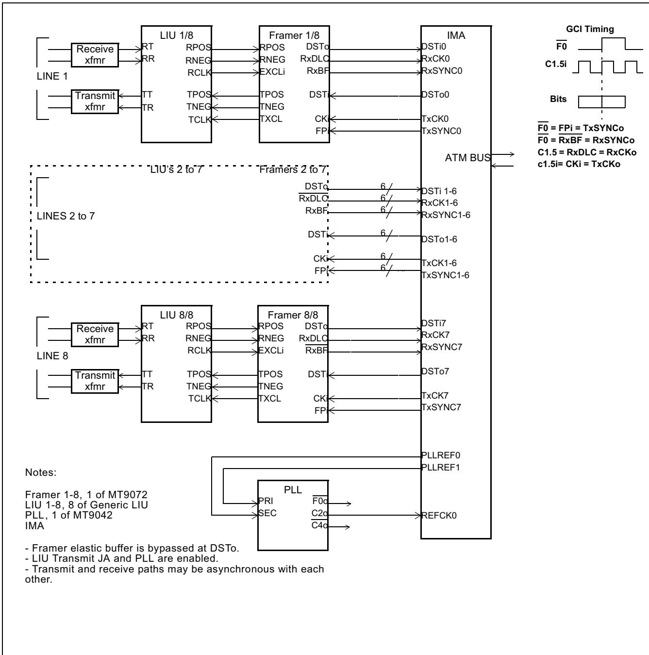
Figure 13 - 8 E1 Links with ATM IMA with Asynchronous ST-BUS Mode
