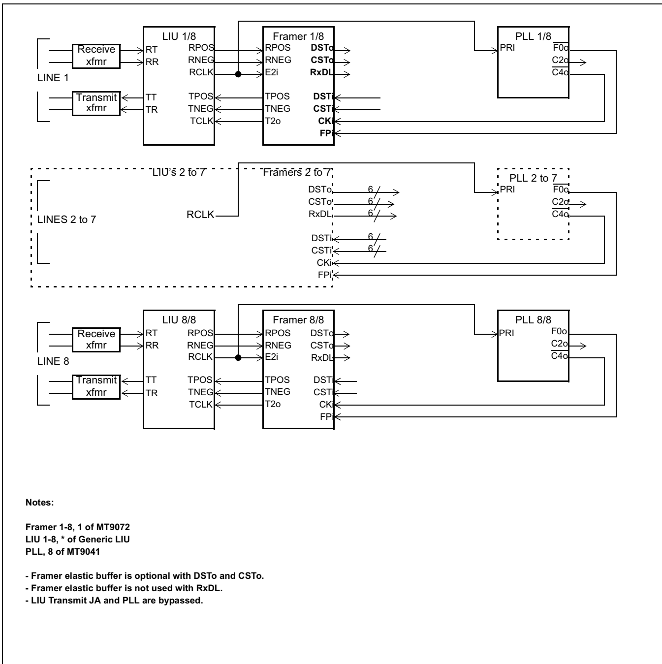
Figure 23 - 8 E1 Links with Asynchronous ST-BUS
