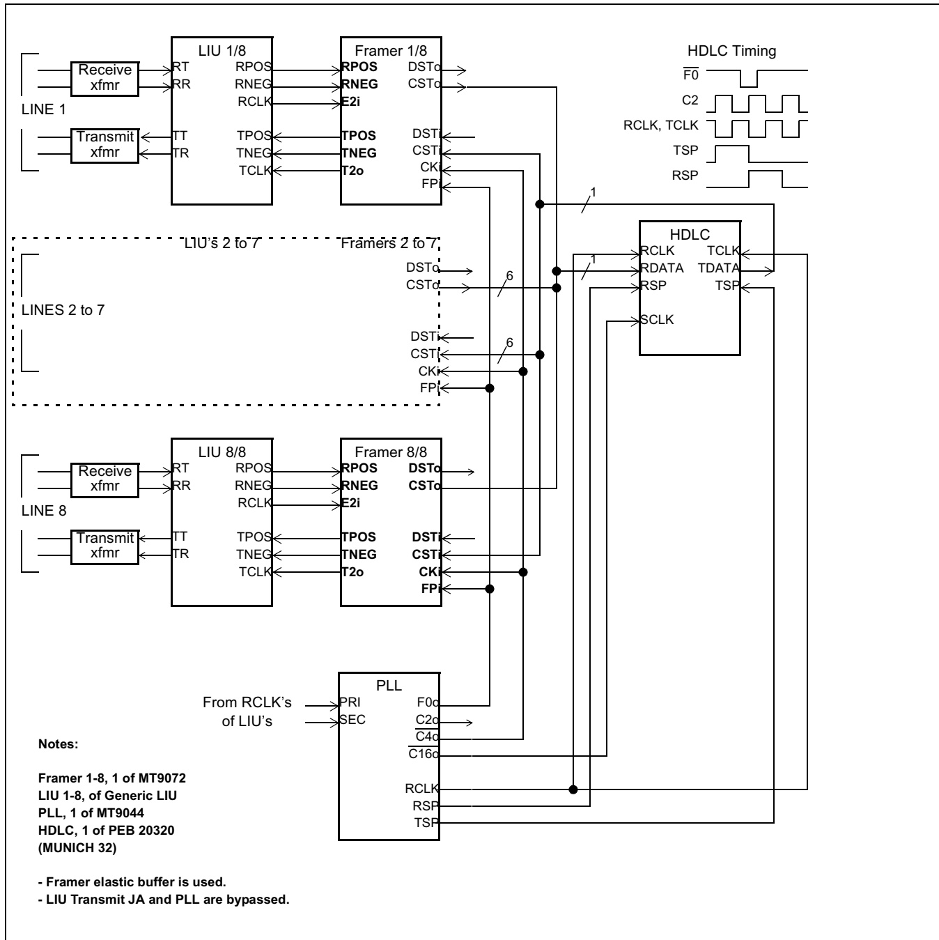
Figure 15 - 8 E1 Links with Synchronous Common Channel Signaling for up to 24 Channels
