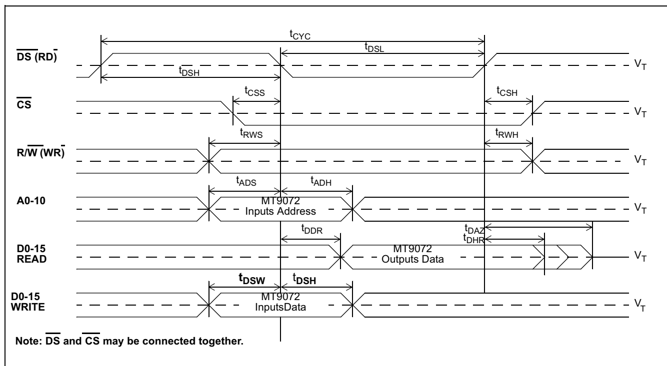
Figure 52 - Motorola Microprocessor Timing
