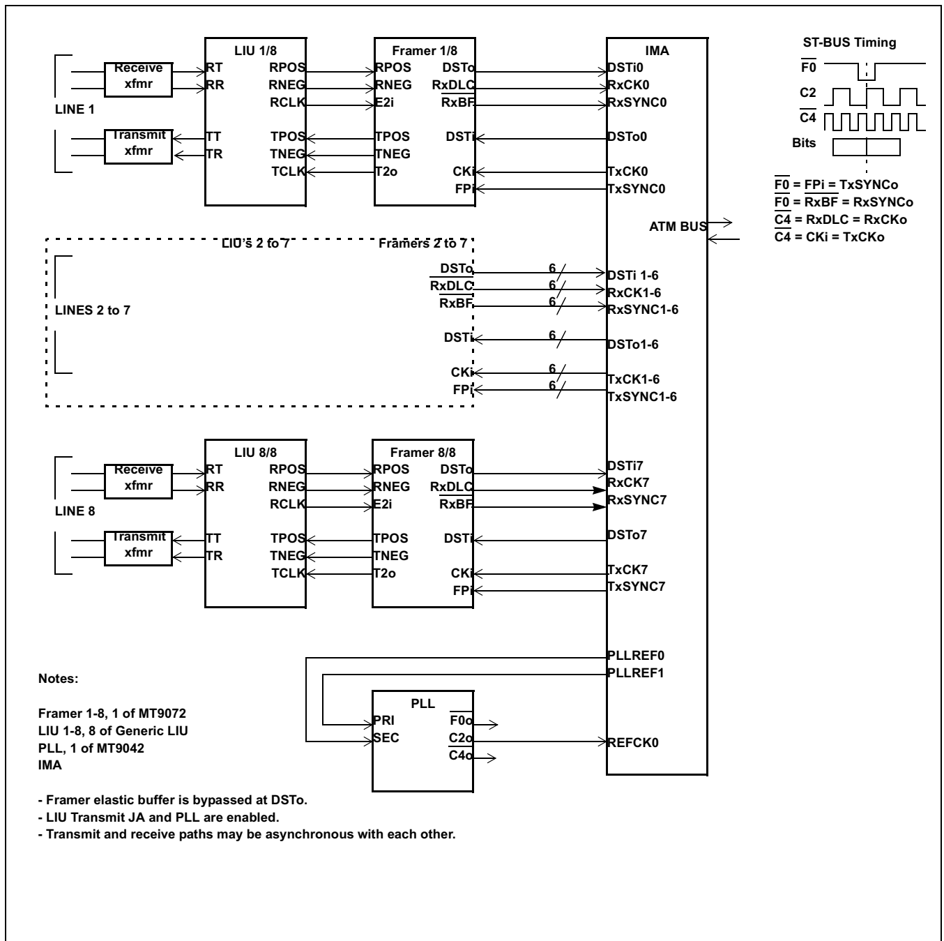
Figure 22 - 8 E1 Links with ATM IMA with Asynchronous ST-BUS Mode
