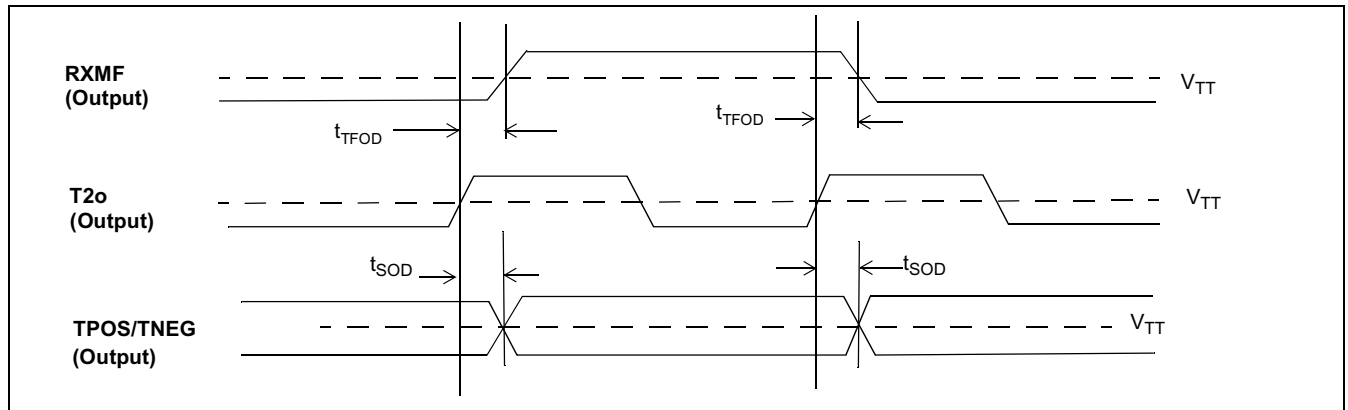
Figure 68 - Receive Multiframe Timing with TX8KEN Set
