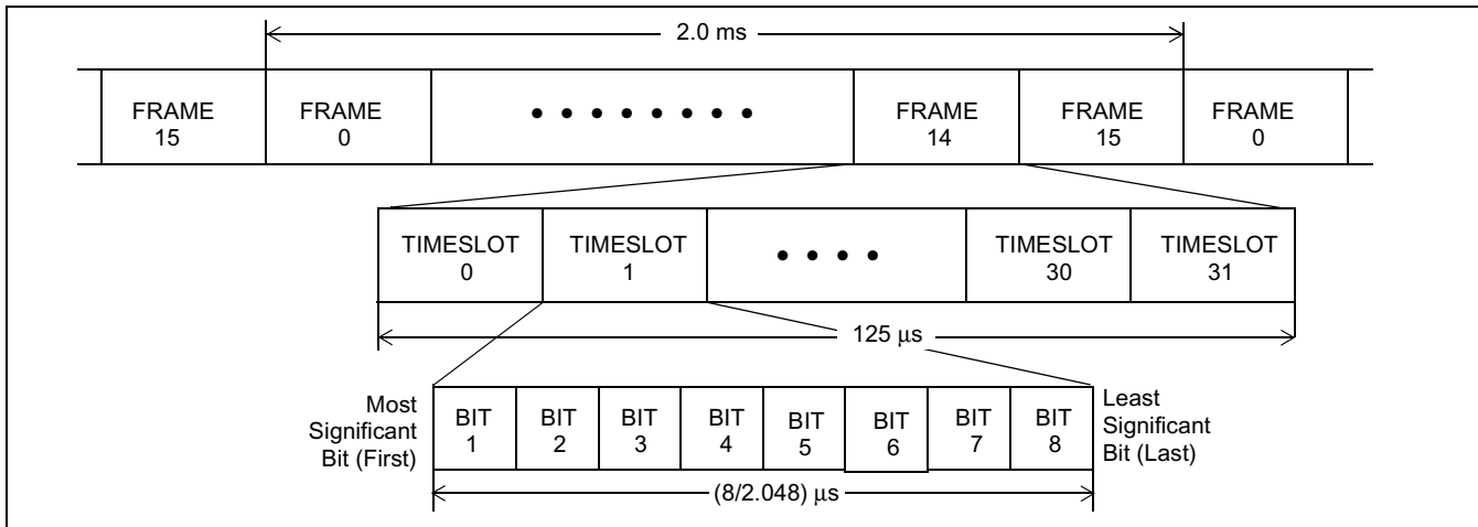
Figure 6 - PCM30 Format (E1)
