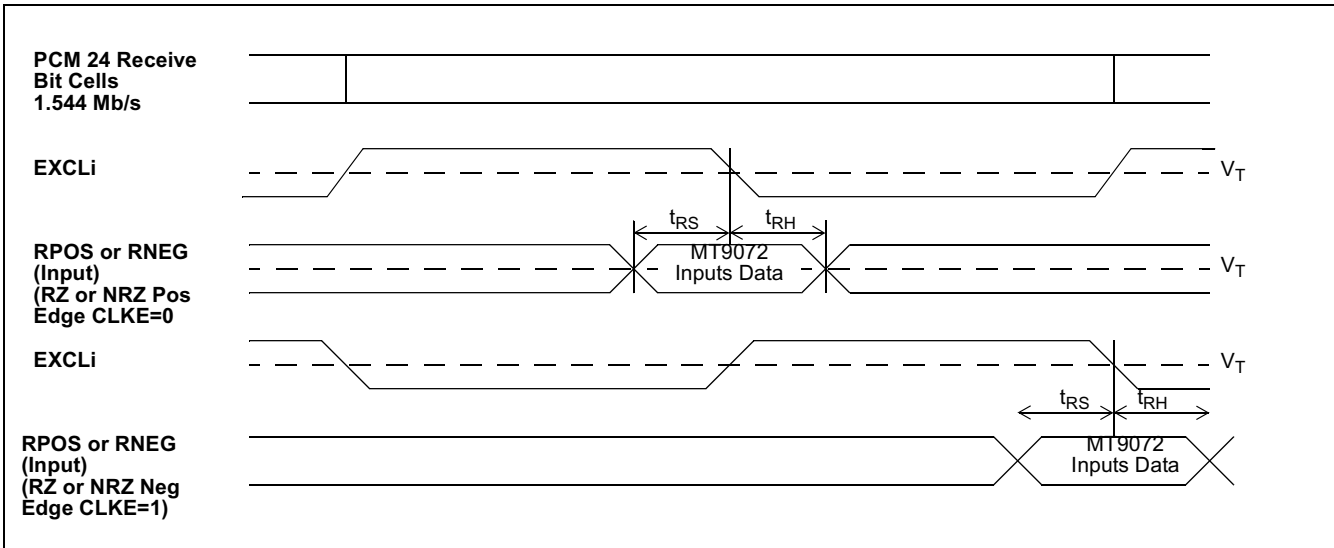
Figure 48 - PCM24 Receive Timing
