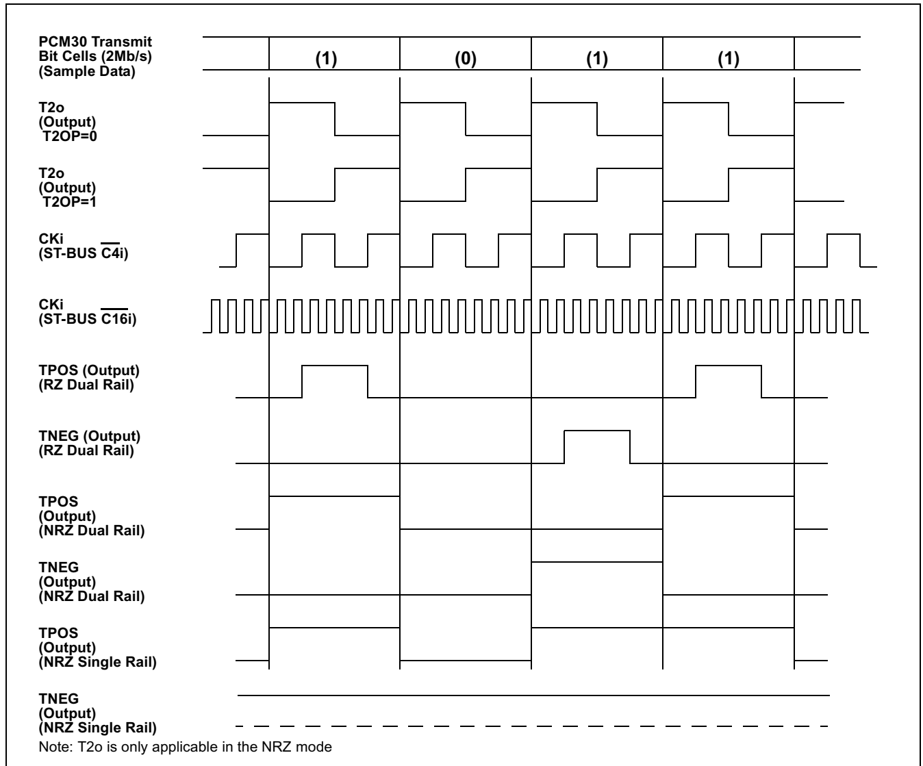
Figure 76 - PCM30 Transmit Functional Timing
