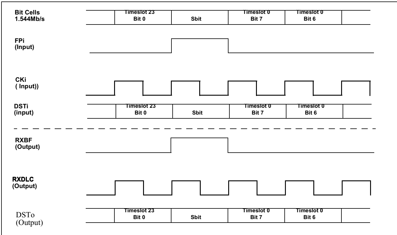
Figure 33 - IMA Functional Timing Diagram
