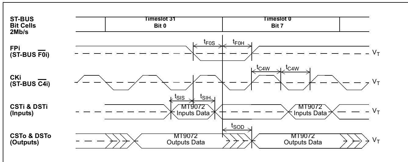
Figure 54 - ST-BUS 2.048Mb/s Timing
