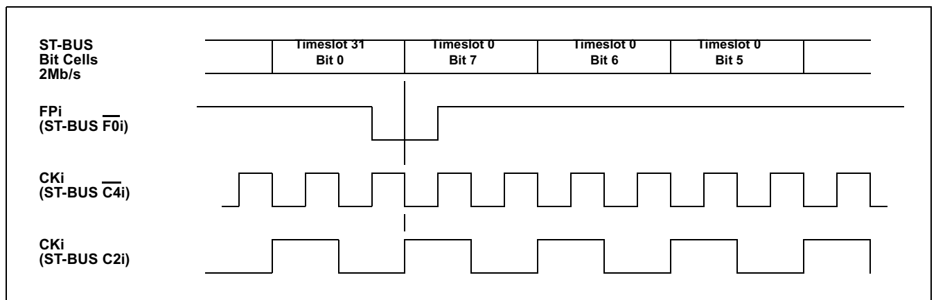
Figure 29 - ST-BUS 2.048Mb/s Functional Timing Diagram
