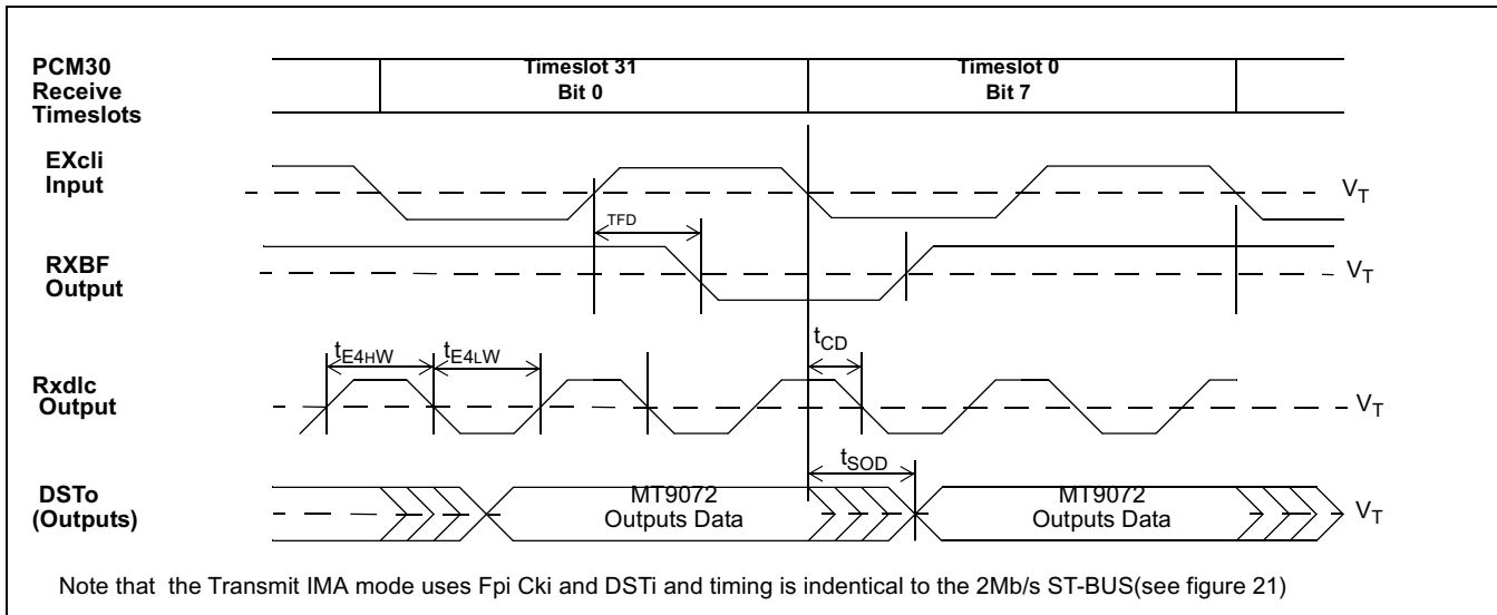
Figure 62 - Receive IMA Timing
