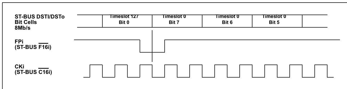
Figure 59 - ST-BUS 8.192Mb/s Functional Timing Diagram for DSTi/DSTo
