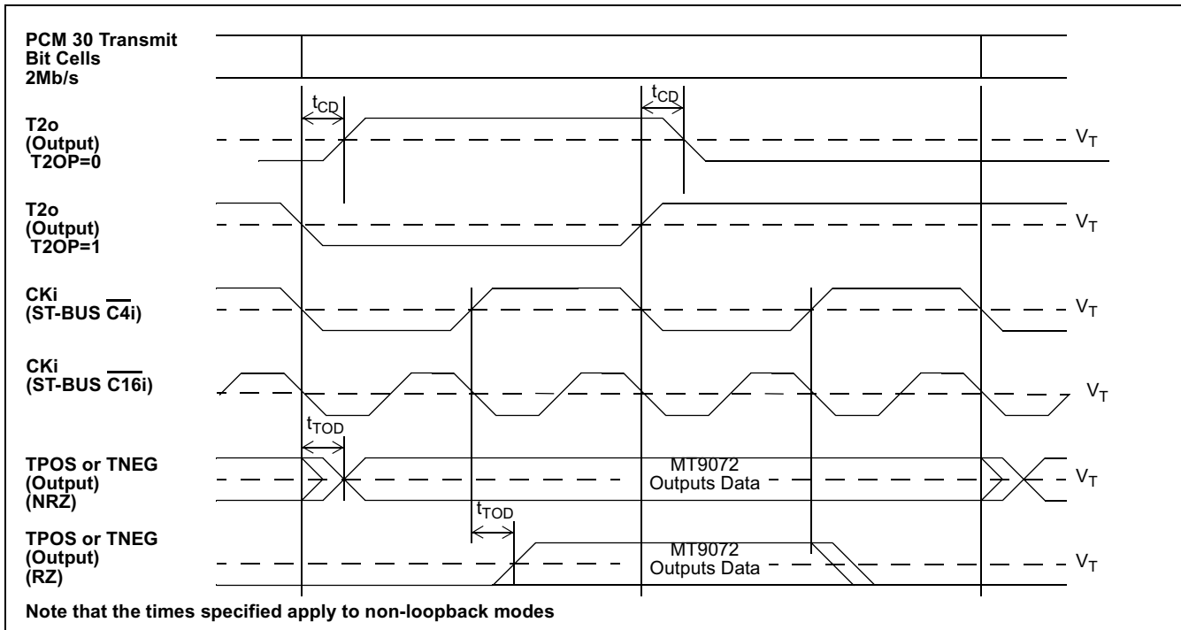
Figure 75 - PCM 30 Transmit Timing
