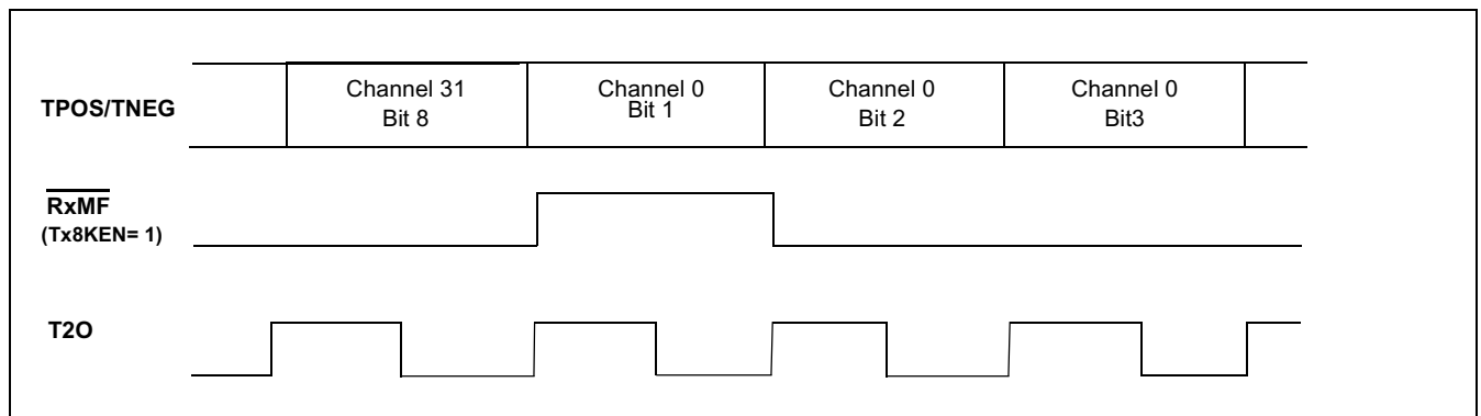
Figure 69 - Receive Multiframe Timing with TX8KEN Set
