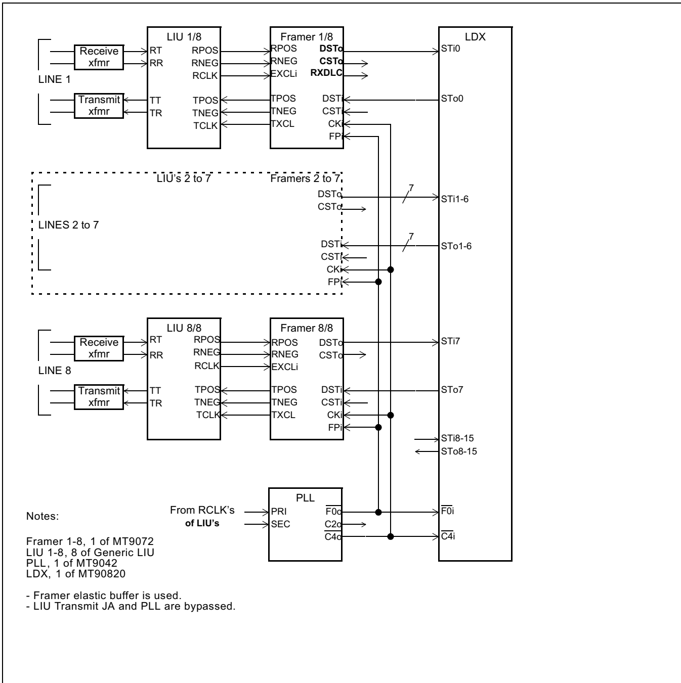
Figure 11 - 8 T1 Links with no JA or PLL in LIU, Slave or Master Mode, Jitter-Free ST-BUS
