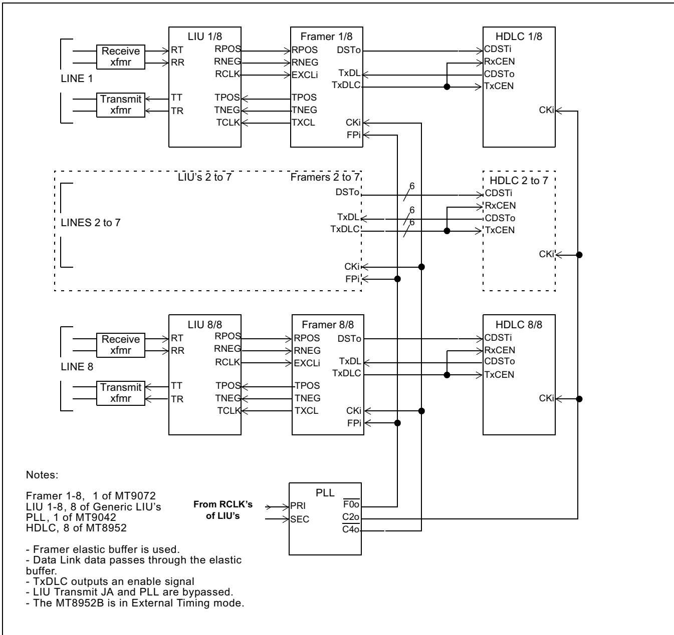
Figure 9 - 8 T1 Links with Synchronous Data Link Signaling
