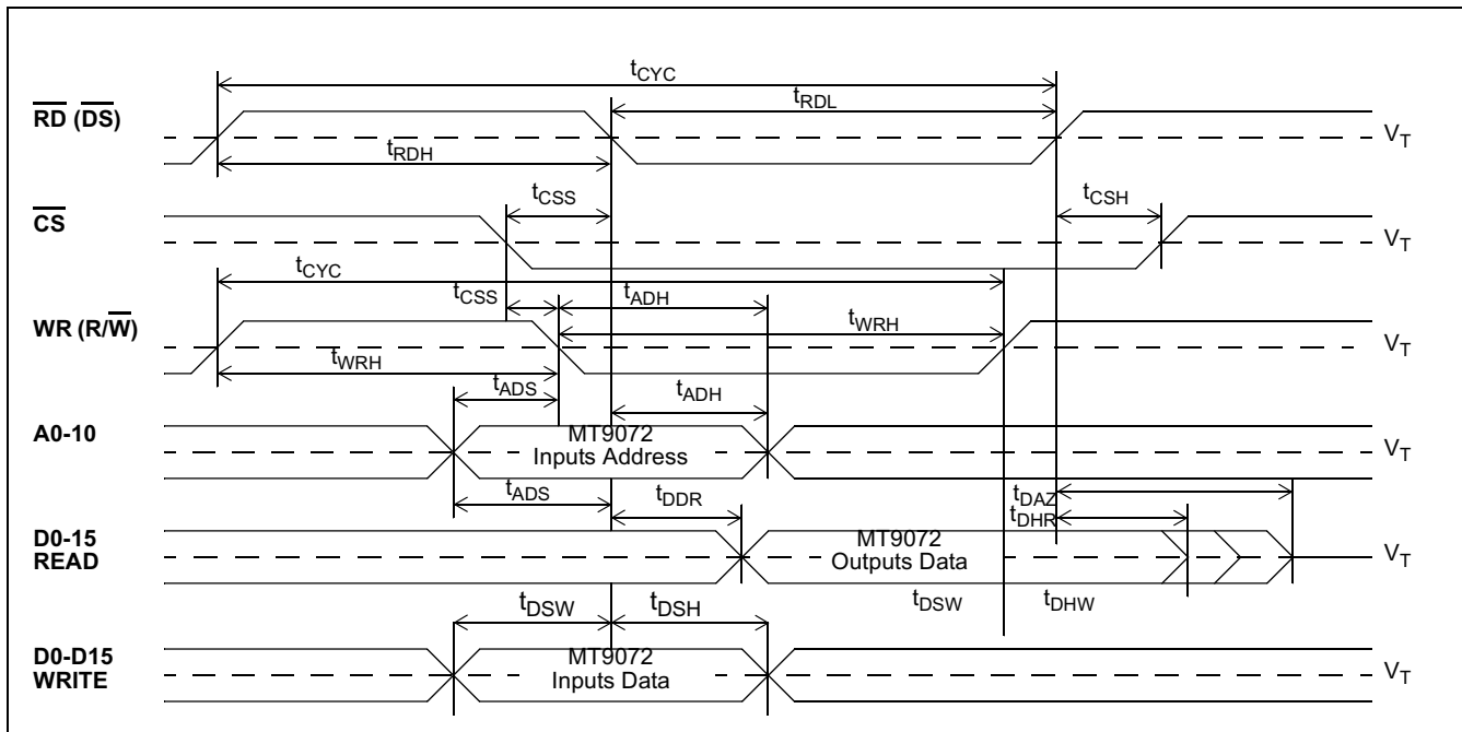
Figure 53 - Intel Microprocessor Timing
