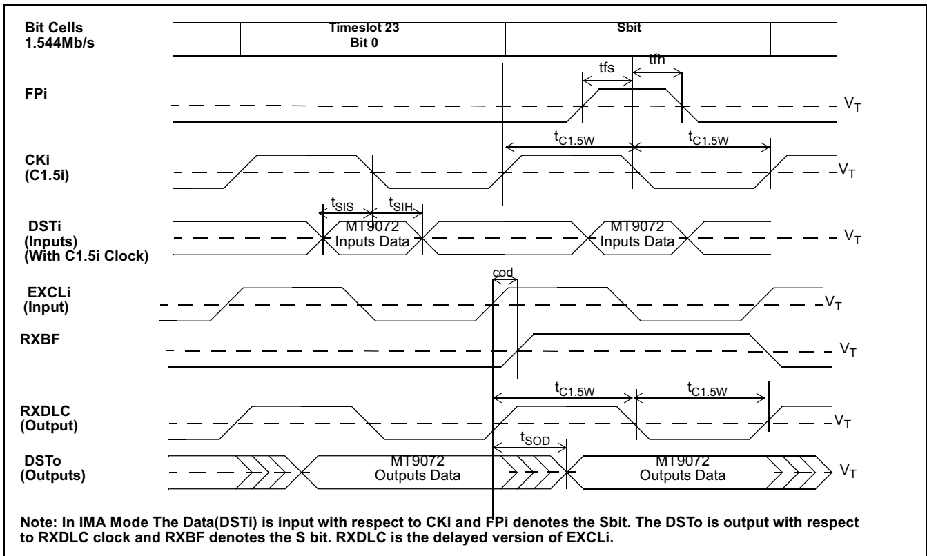
Figure 34 - IMA Mode Timing Diagram
