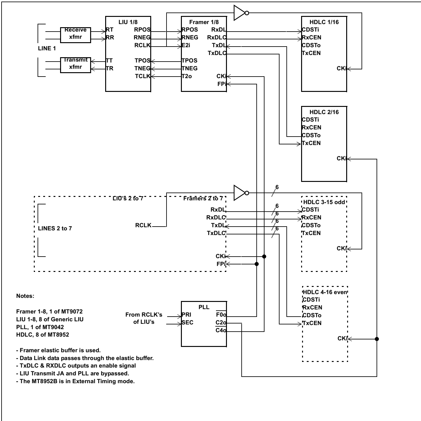
Figure 19 - 8 E1 Links with Asynchronous Data Link Signaling
