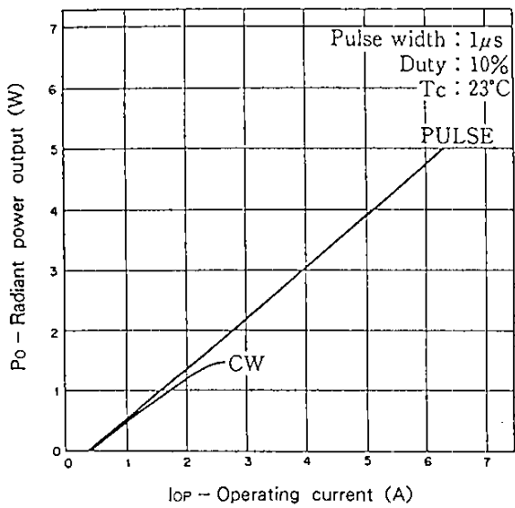
Radiant power output vs. Operating current
