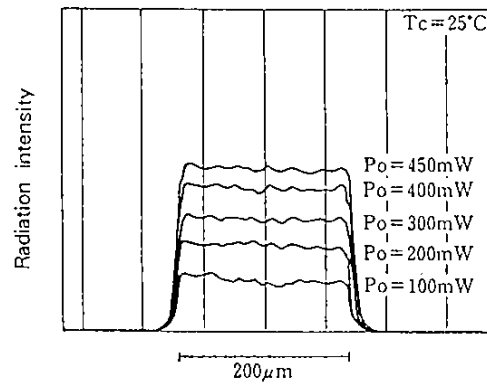
Power dependence of near field pattern
