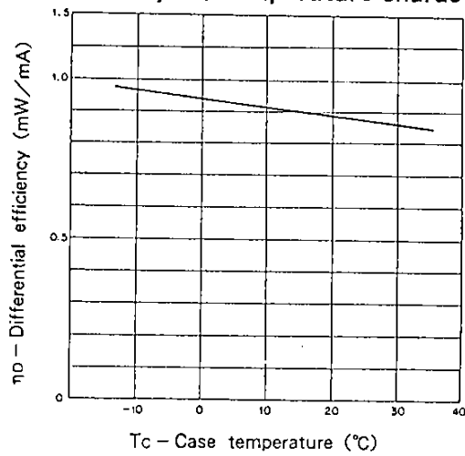
Slope efficiency vs. Temperature characteristics
