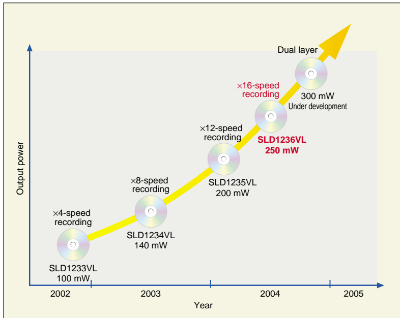
■ Figure 1 DVD Recording Laser Diode Development Trends
