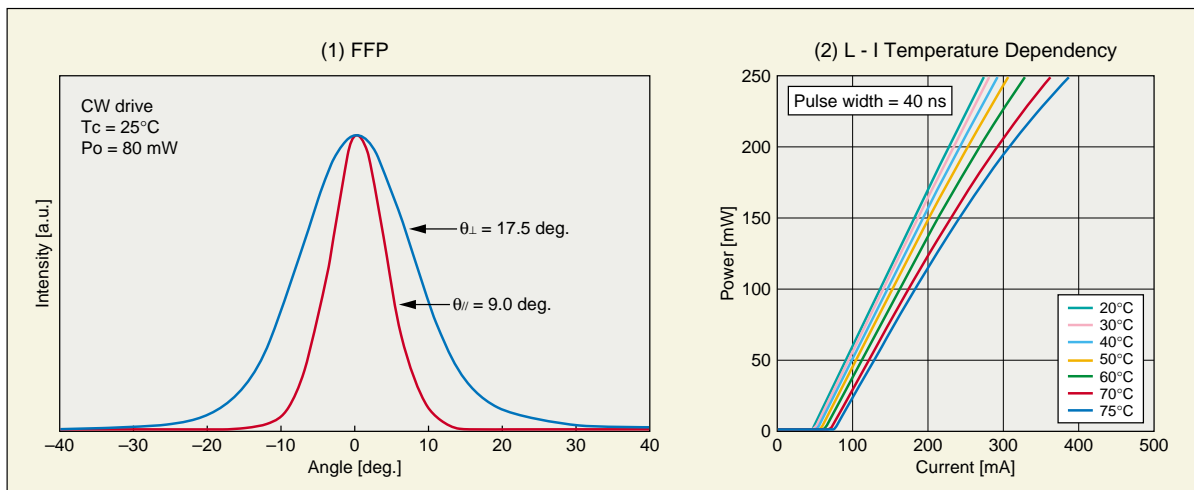
■ Figure 2 SLD1236VL Representative Characteristics
