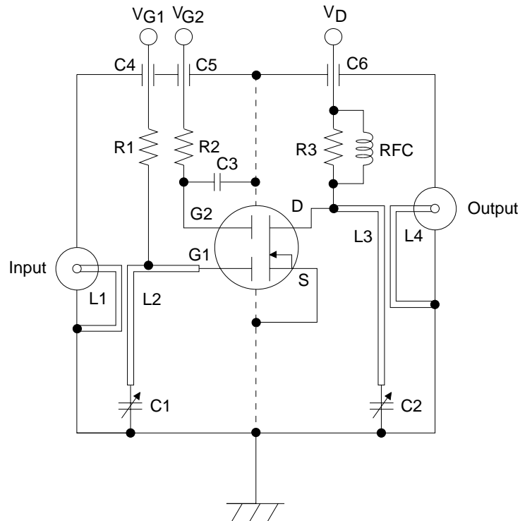
900MHz Power Gain, Noise Test Circuit
