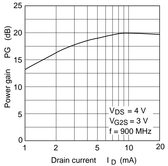
Power Gain vs. Drain Current
