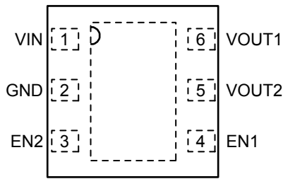
6-Pin 1.6mm x 1.6mm MLF (ML) Top View
