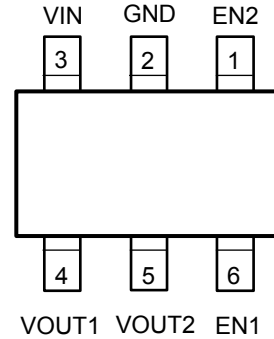
TSOT-23-6 (D6) Top View
