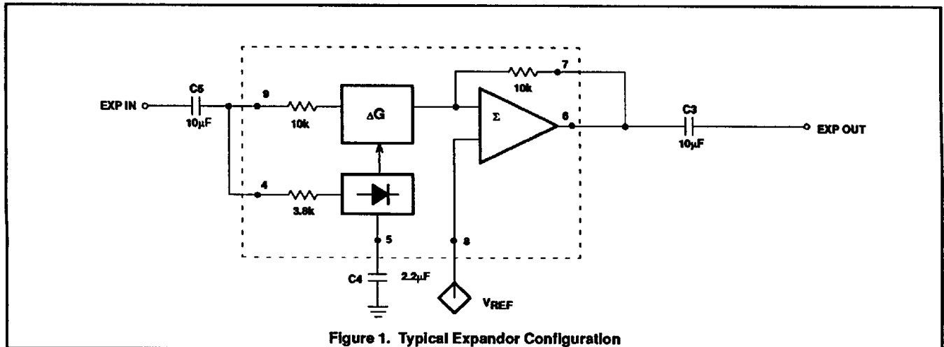
Figure 1. Typical Expandor Configuration
