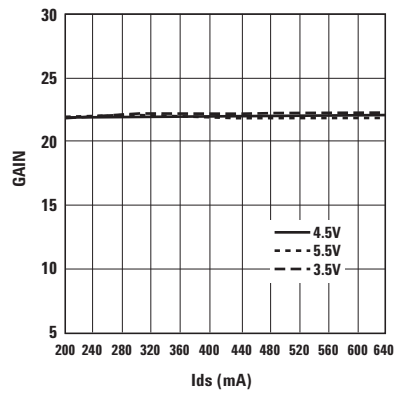
Figure 33. Gain vs. Ids and Vds at 900 MHz.
