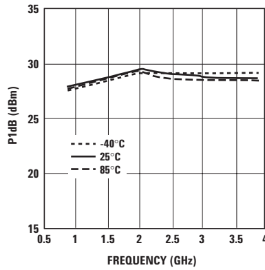
Figure 22. P1dB vs. Temperature and Frequency at optimum OIP3.
