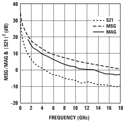
Figure 38. MSG/MAG & |S_{21}|^2 vs. Frequency at 4.5V 360mA.
