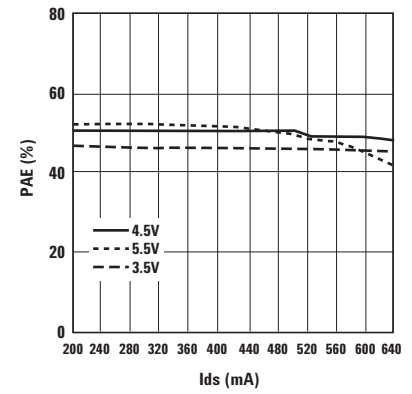
Figure 35. PAE vs. Ids and Vds at 900 MHz.
