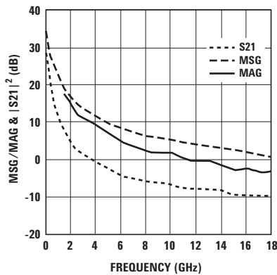
Figure 39. MSG/MAG & |S_{21}|^2 vs. Frequency at 3.5V 280mA.
