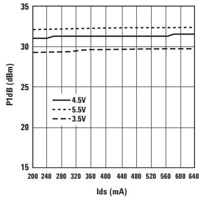
Figure 30. P1dB vs. Ids and Vds at 2 GHz.
