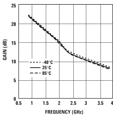
Figure 25. Gain vs. Temperature and Frequency at optimum P1dB.
