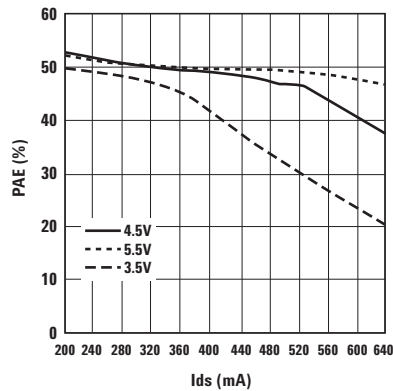
Figure 18. PAE vs. Ids and Vds at 2 GHz.
