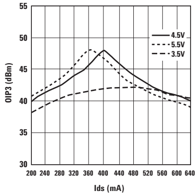
Figure 12. OIP3 vs. Ids and Vds at 2 GHz.
