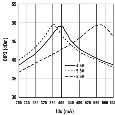
Figure 13. OIP3 vs. Ids and Vds at 900 MHz.
