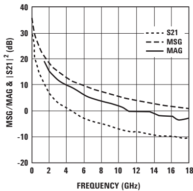
Figure 42. MSG/MAG & |S_{21}|^2 vs. Frequency at 5.5V 280mA.
