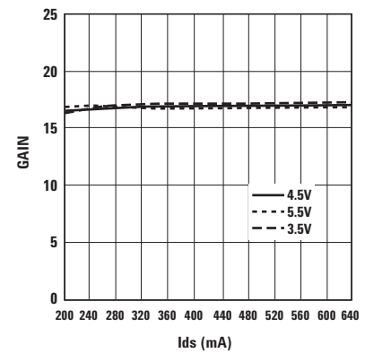
Figure 17. Gain vs. Ids and Vds at 900 MHz.
