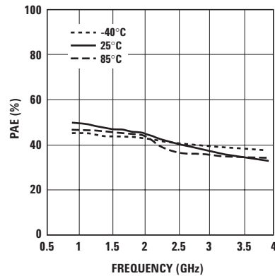
Figure 27. PAE vs. Temperature and Frequency at optimum P1dB.
