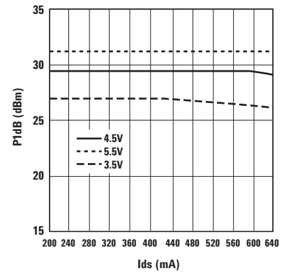
Figure 14. P1dB vs. Ids and Vds at 2 GHz.
