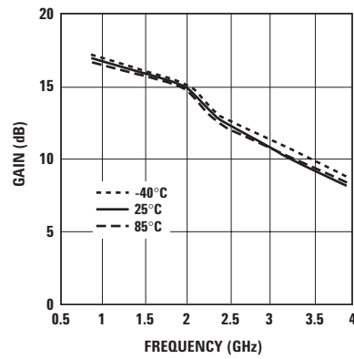
Figure 24. Gain vs. Temperature and Frequency at optimum OIP3.
