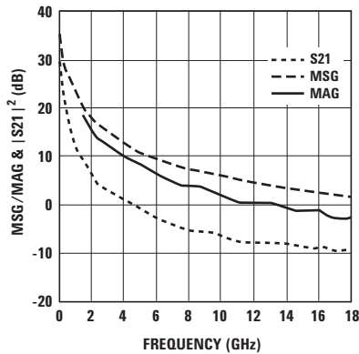
Figure 37. MSG/MAG & |S_{21}|^2 vs. Frequency at 4.5V 200mA.
