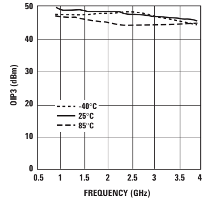
Figure 20. OIP3 vs. Temperature and Frequency at optimum OIP3.
