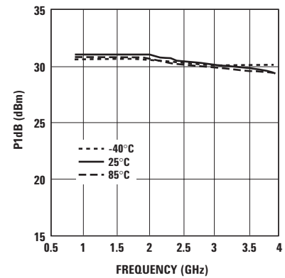
Figure 23. P1dB vs. Temperature and Frequency at optimum P1dB.
