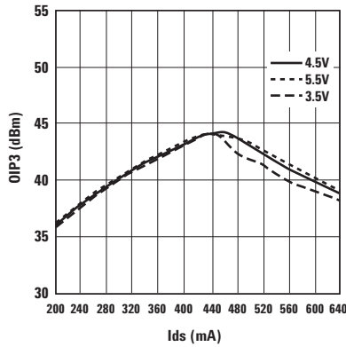
Figure 28. OIP3 vs. Ids and Vds at 2 GHz.
