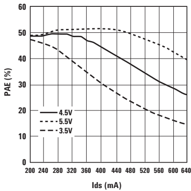
Figure 19. PAE vs. Ids and Vds at 900 MHz.
