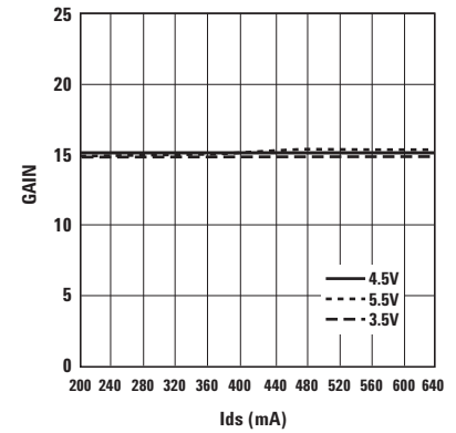
Figure 32. Gain vs. Ids and Vds at 2 GHz.
