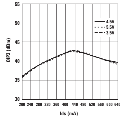
Figure 29. OIP3 vs. Ids and Vds at 900 MHz.
