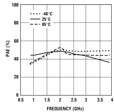
Figure 26. PAE vs. Temperature and Frequency at optimum OIP3.
