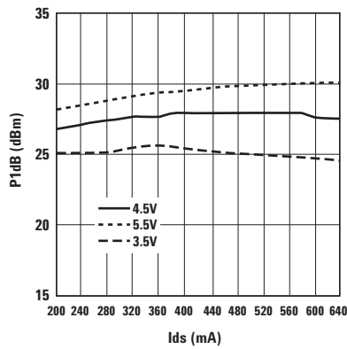
Figure 15. P1dB vs. Ids and Vds at 900 MHz.
