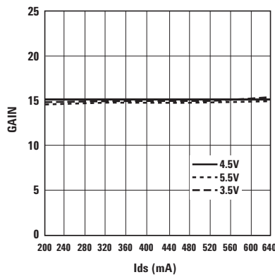
Figure 16. Gain vs. Ids and Vds at 2 GHz.
