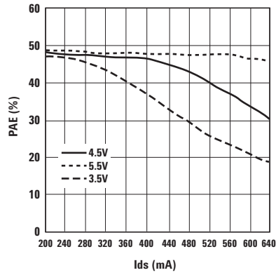
Figure 11. PAE vs. Ids and Vds at 2 GHz.
