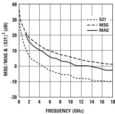
Figure 44. MSG/MAG & |S_{21}|^2 vs. Frequency at 5.5V 360mA.
