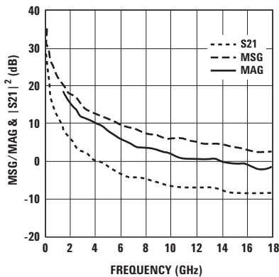
Figure 40. MSG/MAG & |S_{21}|^2 vs. Frequency at 3.5V 200mA.
