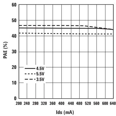
Figure 34. PAE vs. Ids and Vds at 2 GHz.
