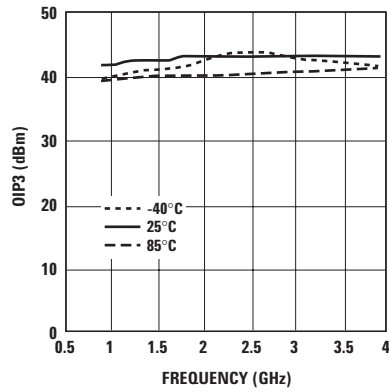
Figure 21. OIP3 vs. Temperature and Frequency at optimum P1dB.
