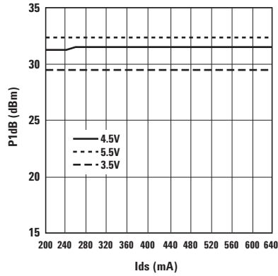
Figure 31. P1dB vs. Ids and Vds at 900 MHz.
