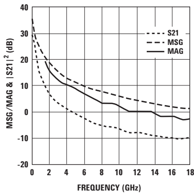
Figure 43. MSG/MAG & |S_{21}|^2 vs. Frequency at 5.5V 200mA.
