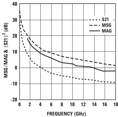
Figure 41. MSG/MAG & |S_{21}|^2 vs. Frequency at 3.5V 360mA.
