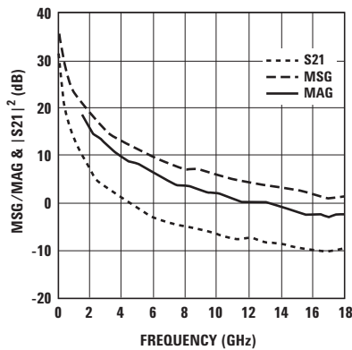
Figure 36. MSG/MAG & |S_{21}|^2 vs. Frequency at 4.5V 280mA.
