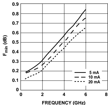
Figure 12. F_{min} vs. Frequency and Current at 2V.
