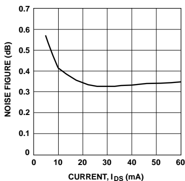
Figure 9. Noise Figure vs. I_d at 2V, 900 MHz.
