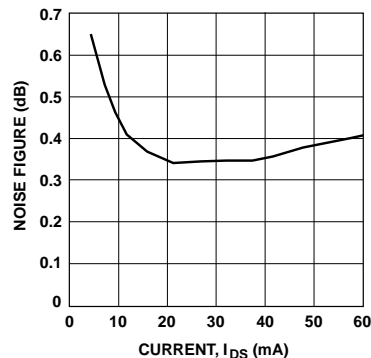
Figure 8. Noise Figure vs. I_d at 2V, 2 GHz.
