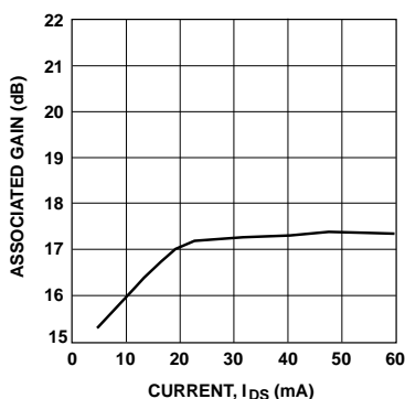
Figure 10. Associated Gain vs. I_d at 2V, 2 GHz.
