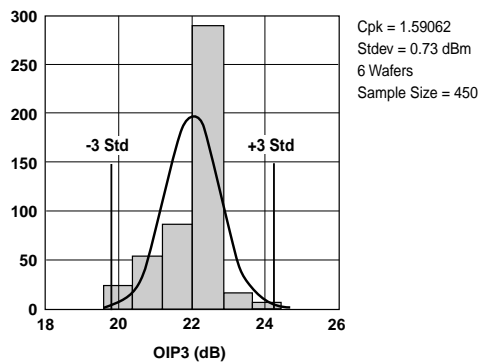
Figure 2. OIP3 @ 2 GHz, 2 V, 10 mA. LSL=18.5, Nominal=21.99, USL=26.0
