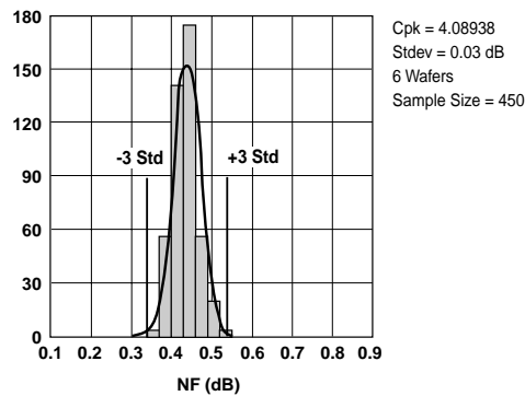
Figure 3. NF @ 2 GHz, 2 V, 10 mA. LSL=0, Nominal=0.44, USL=0.85
