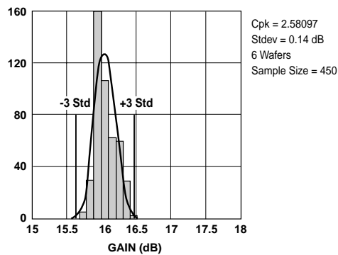
Figure 4. Gain @ 2 GHz, 2 V, 10 mA. LSL=15.0, Nominal=16.06, USL= 18.0
