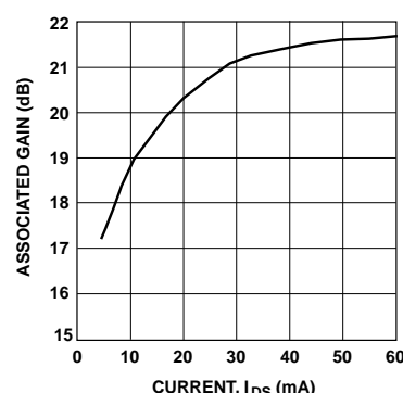
Figure 11. Associated Gain vs. I_d at 2V, 900 MHz.
