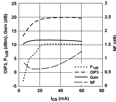
Figure 17. OIP3, P_{1dB} , NF and Gain vs. Bias [1] (Active Bias, 2V, 5.8 GHz).
