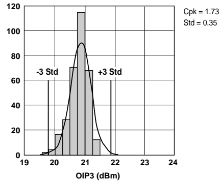
Figure 2. OIP3 @ 2 GHz, 2 V, 15 mA. LSL=19.0, Nominal=20.9, USL=23.0
