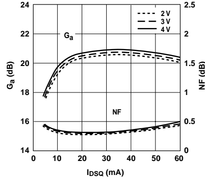
Figure 9. NF and G_a vs. Bias at 900MHz. [1]
