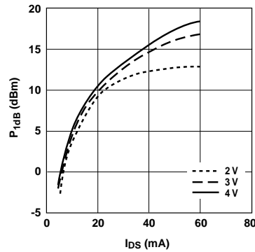
Figure 11. P_{1dB} vs. Bias (Active Bias)
