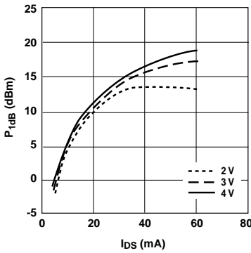
Figure 10. P_{1dB} vs. Bias (Active Bias)
