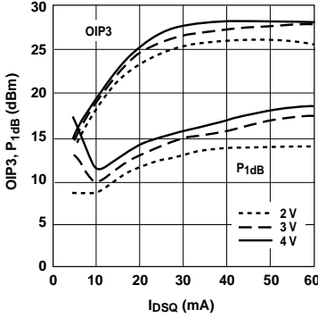
Figure 6. OIP3 and P_{1dB} vs. Bias at 2GHz. [1,2]
