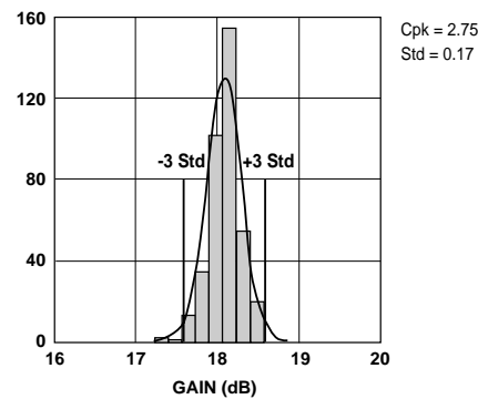
Figure 4. Gain @ 2 GHz, 2 V, 15 mA. LSL=16.5, Nominal=18.0, USL=19.5
