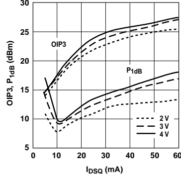
Figure 7. OIP3 and P_{1dB} vs. Bias at 900MHz. [1,2]
