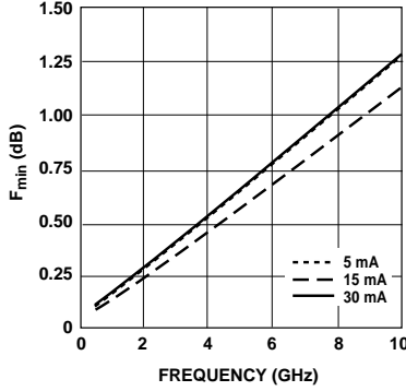
Figure 12. F_{min} vs. Frequency and Current at 2V.
