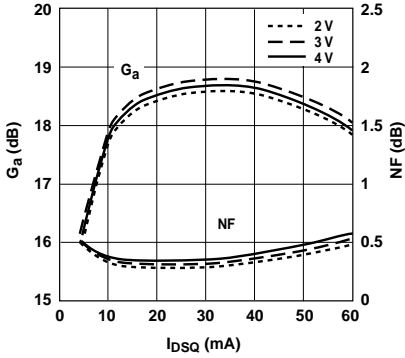
Figure 8. NF and G_a vs. Bias at 2GHz. [1]
