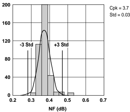
Figure 3. NF @ 2 GHz, 2 V, 15 mA. LSL=0.2, Nominal=0.37, USL=0.7
