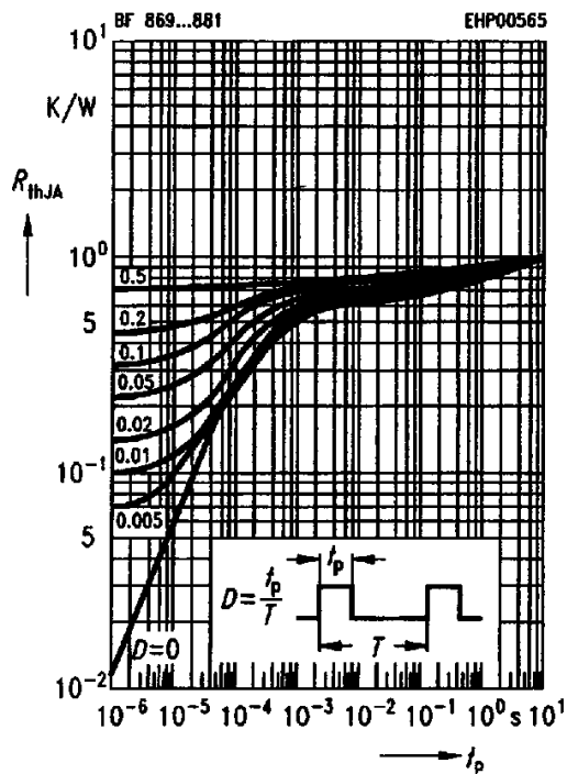
Permissible pulse load R_{thJA} = f(t_p)
