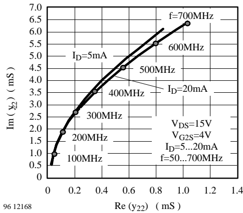
Figure 10. Short Circuit Output Admittance
