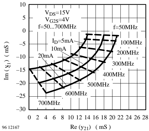
Figure 9. Short Circuit Forward Transfer Admittance
