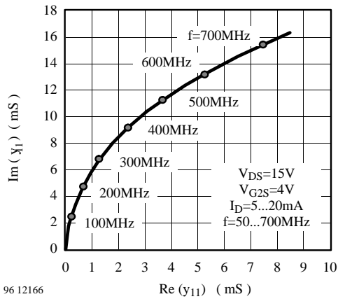
Figure 8. Short Circuit Input Admittance
