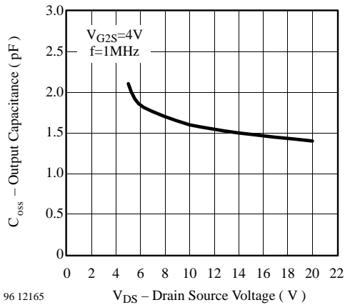
Figure 7. Output Capacitance vs. Drain Source Voltage
