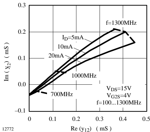
Figure 11. Short Circuit Reverse Transfer Admittance
