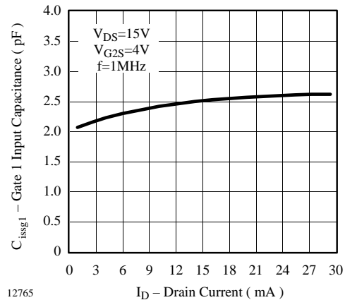
Figure 5. Gate 1 Input Capacitance vs. Drain Current
