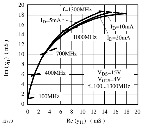
Figure 10. Short Circuit Input Admittance
