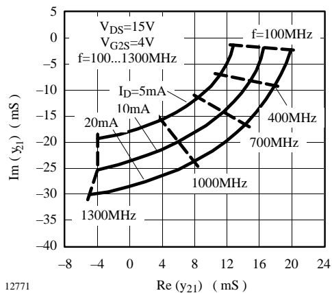
Figure 12. Short Circuit Forward Transfer Admittance
