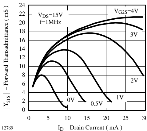
Figure 9. Forward Transadmittance vs. Drain Current
