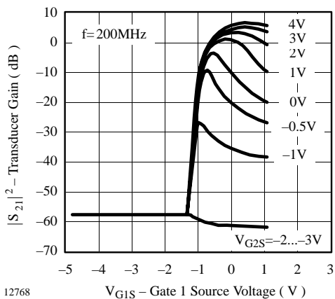
Figure 8. Transducer Gain vs. Gate 1 Source Voltage
