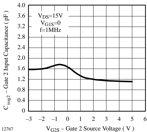
Figure 7. Gate 2 Input Capacitance vs. Gate 2 Source Voltage
