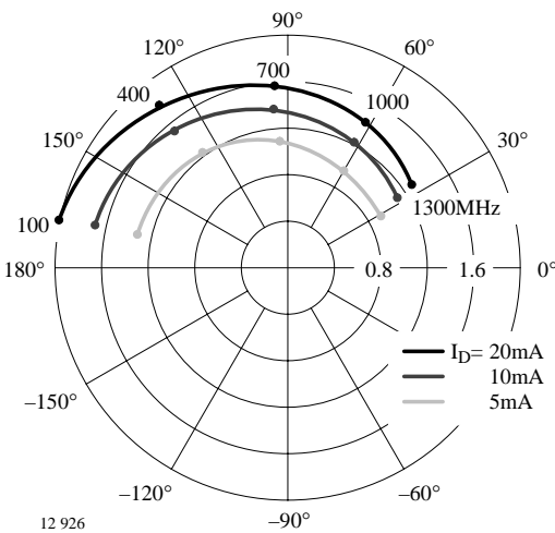
Figure 15. Forward transmission coefficient
