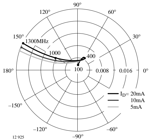
Figure 16. Reverse transmission coefficient
