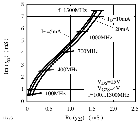
Figure 13. Short Circuit Output Admittance
