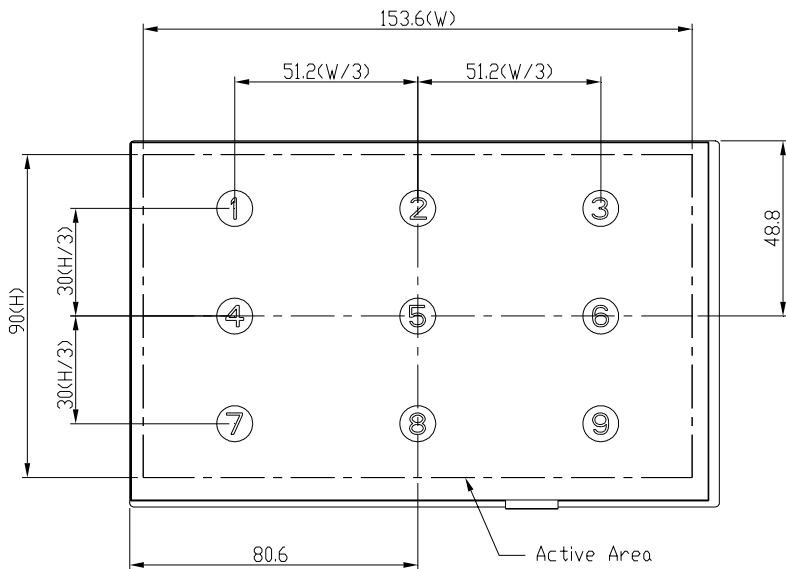
Fig9-1 Measuring point
