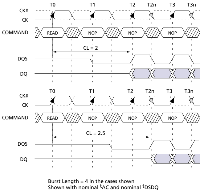
CAS Latency Diagram
